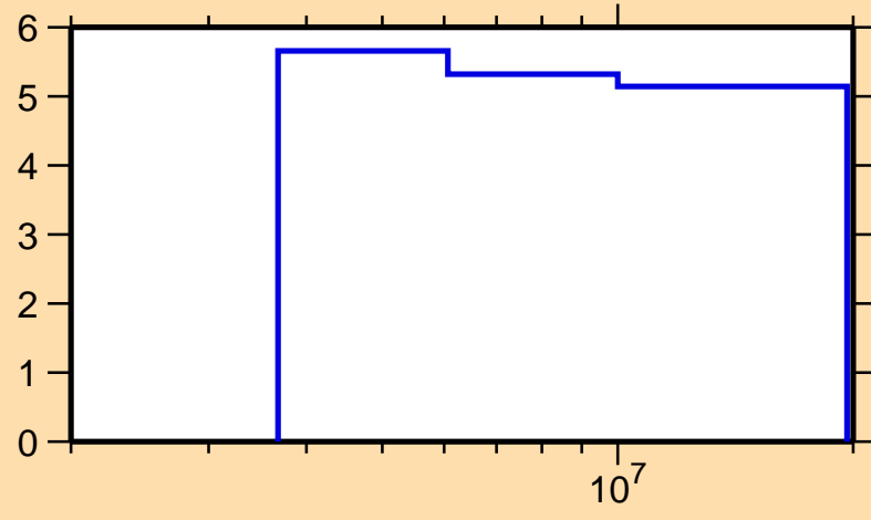
\Delta\sigma/\sigma vs. E for ^{52}\text{Cr}(n,n\text{onel.})
