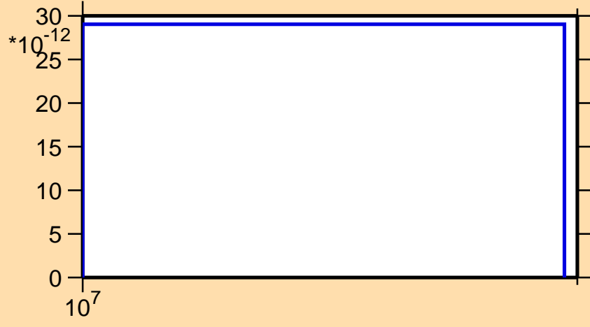
\sigma vs. E for ^{52}\text{Cr}(n,\text{pd})
