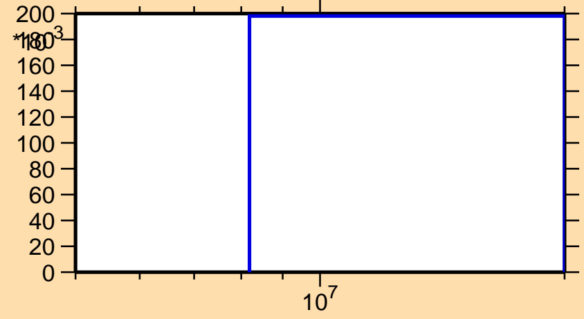
\sigma vs. E for ^{52}\text{Cr}(n,2n)
