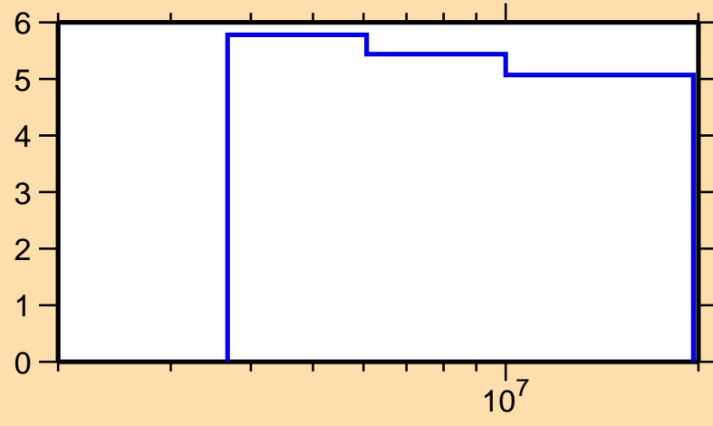
\Delta\sigma/\sigma vs. E for ^{53}\text{Cr}(n,n\text{onel.})
