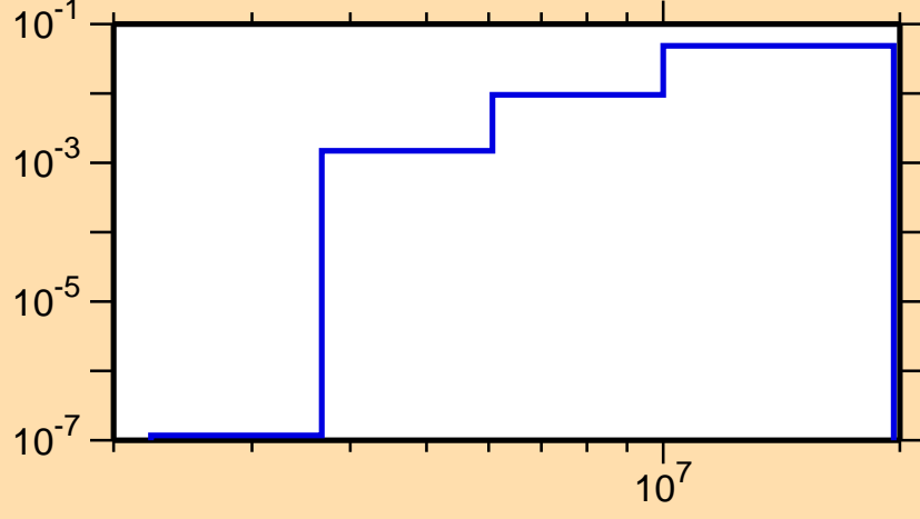
\sigma vs. E for ^{53}\text{Cr}(n,p)
