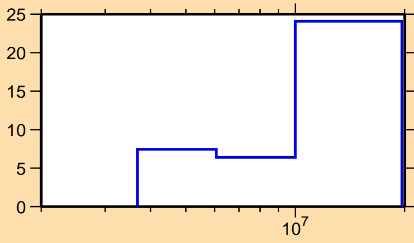
\Delta\sigma/\sigma vs. E for ^{53}\text{Cr}(n,ncont.)
