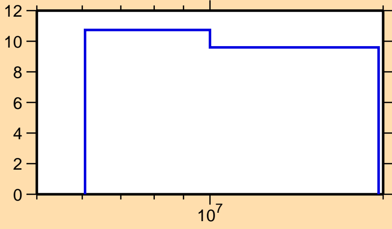
\Delta\sigma/\sigma vs. E for ^{53}\text{Cr}(n,2n)
