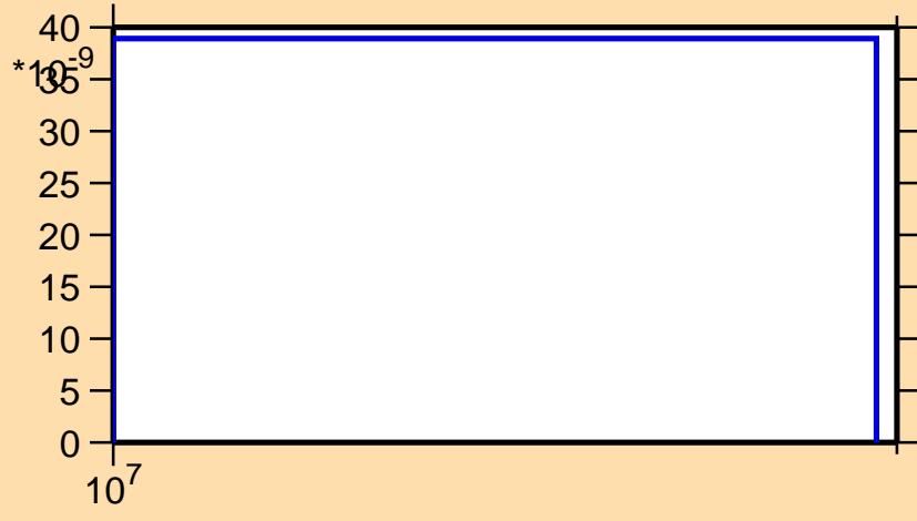
\sigma vs. E for ^{53}\text{Cr}(n,\text{nd})
