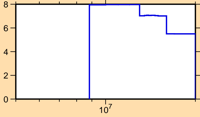
\Delta\sigma/\sigma vs. E for ^{54}\text{Cr}(n,tot.)
