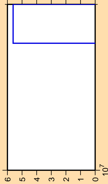
\Delta\sigma/\sigma vs. E for ^{54}\text{Cr}(n,\text{nd})
