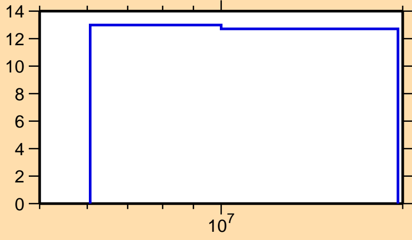
\Delta\sigma/\sigma vs. E for ^{54}\text{Cr}(n,el.)
