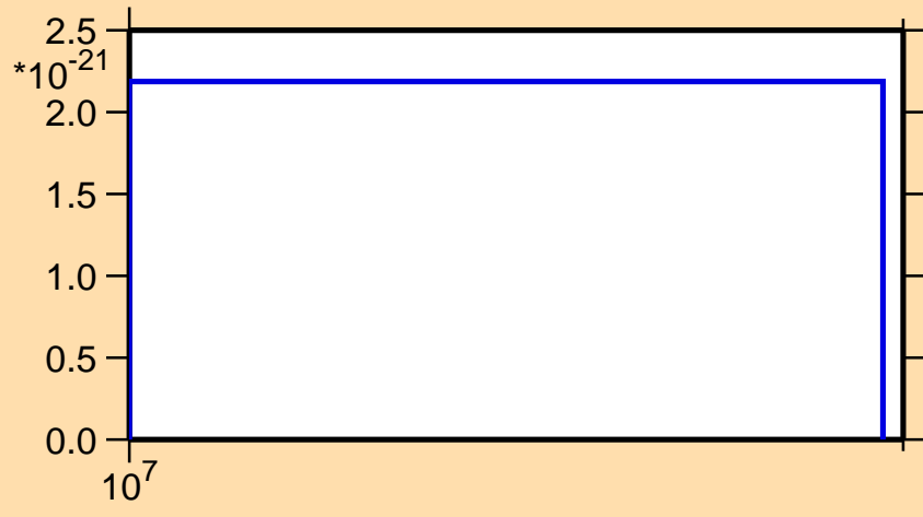
\sigma vs. E for ^{54}\text{Cr}(\text{mt117})
