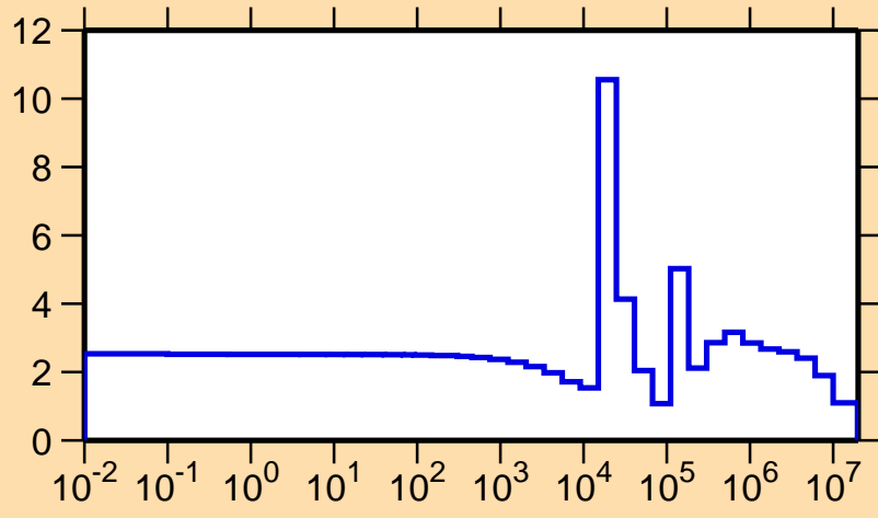
\sigma vs. E for ^{54}\text{Cr}(n,\text{el.})
