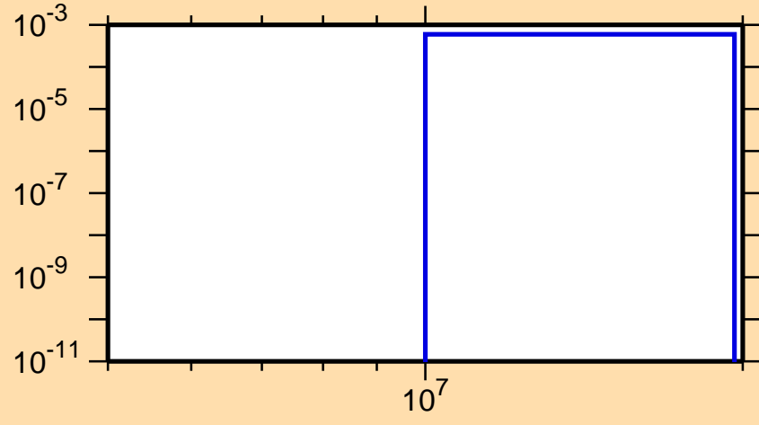
\sigma vs. E for ^{54}\text{Cr}(n,\alpha)
