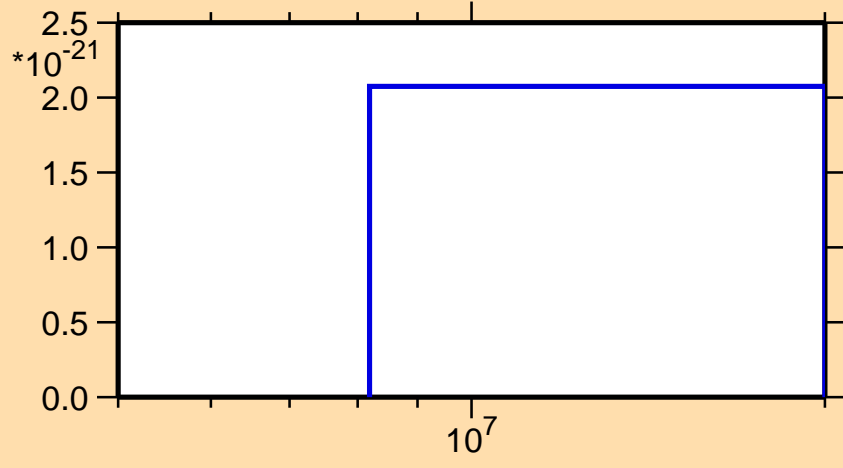
\sigma vs. E for ^{54}\text{Cr}(\text{mt117})
