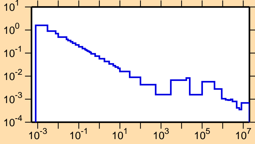
\sigma vs. E for ^{54}\text{Cr}(n,\gamma)
