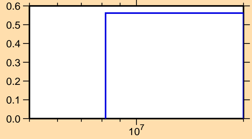
\sigma vs. E for ^{54}\text{Cr}(n,2n)
