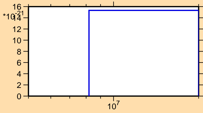
\sigma vs. E for ^{54}\text{Cr}(n,2n\alpha)
