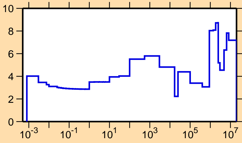
\Delta\sigma/\sigma vs. E for ^{54}\text{Cr}(n,\text{tot.})
