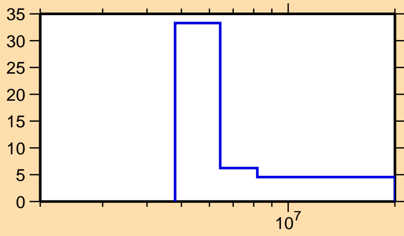
\Delta\sigma/\sigma vs. E for ^{55}\text{Cr}(n,2n)
