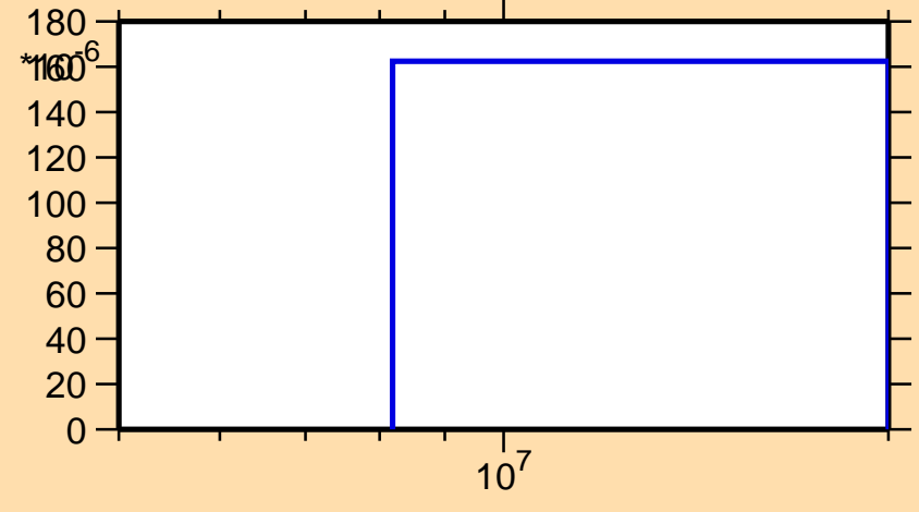
\sigma vs. E for ^{55}\text{Cr}(n,np)
