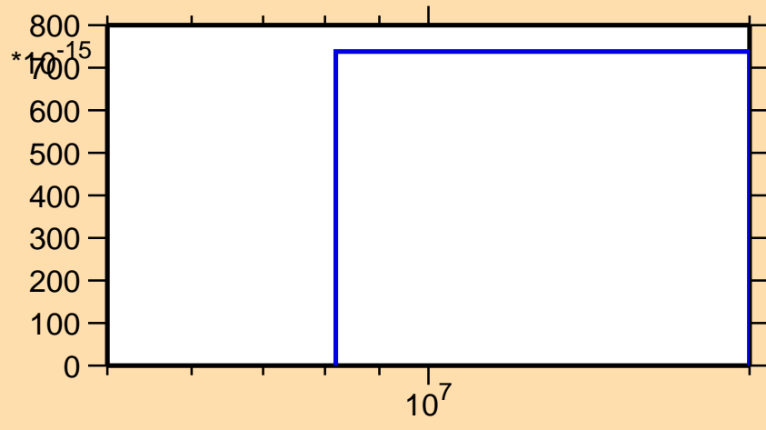
\sigma vs. E for ^{55}\text{Cr}(n,2np)
