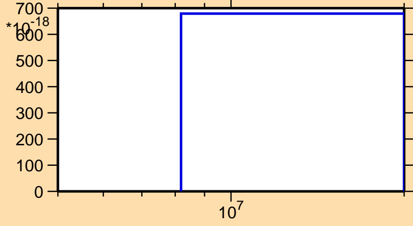
\sigma vs. E for ^{55}\text{Cr}(n,nt)
