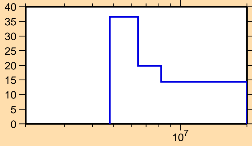
\Delta\sigma/\sigma vs. E for ^{55}\text{Cr}(n,p)
