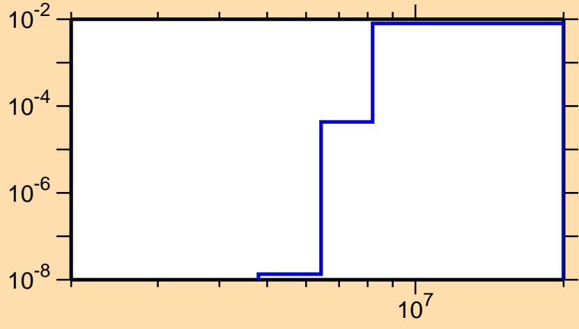
\sigma vs. E for ^{55}\text{Cr}(n,p)
