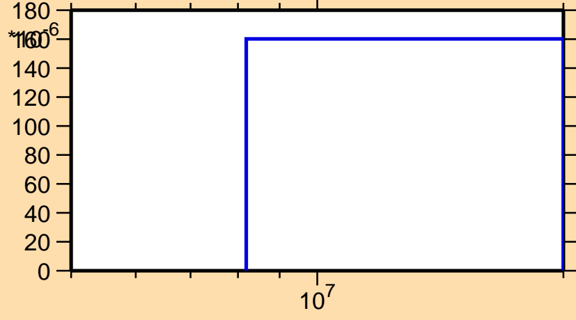
\sigma vs. E for ^{55}\text{Cr}(n,3n)
