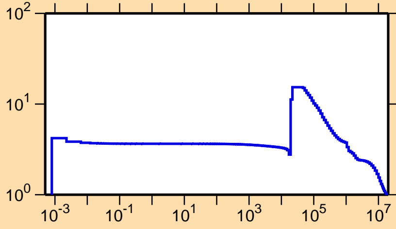
\sigma vs. E for ^{56}\text{Cr}(n,\text{el.})
