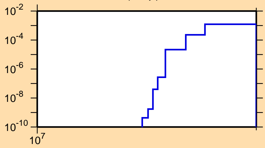
\sigma vs. E for ^{56}\text{Cr}(n,np)
