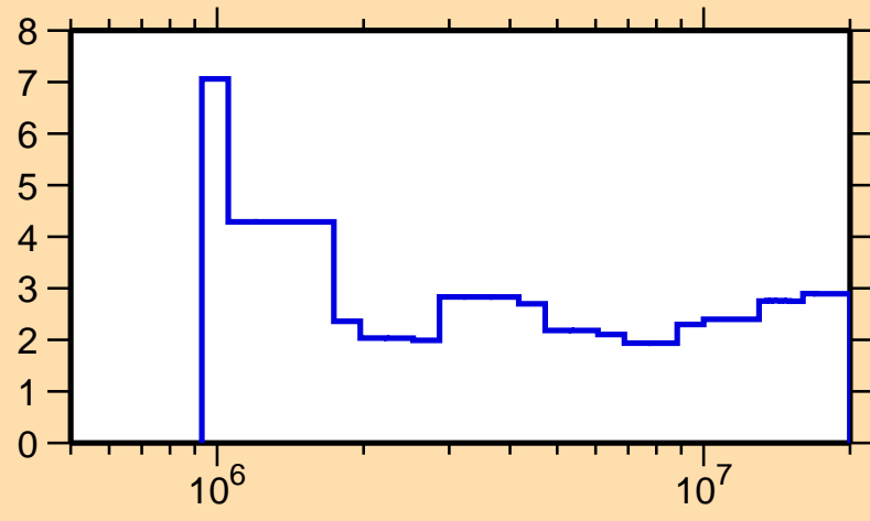
\Delta\sigma/\sigma vs. E for ^{56}\text{Cr}(n,\text{nonel.})
