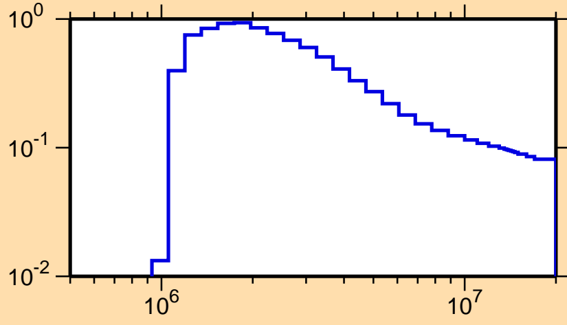
\sigma vs. E for ^{56}\text{Cr}(n,n_1)
