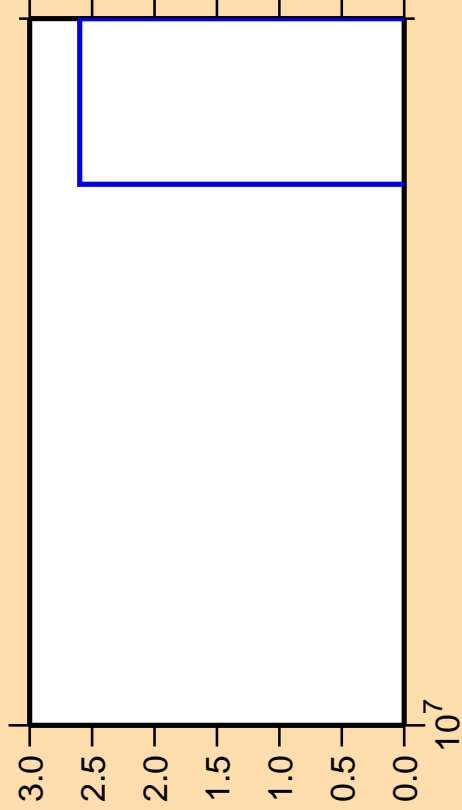
\Delta\sigma/\sigma vs. E for ^{56}\text{Cr}(n,\text{nd})
