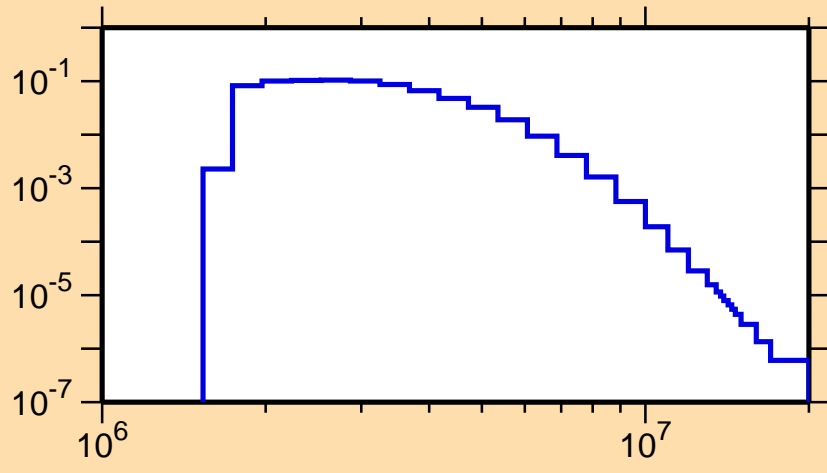
\sigma vs. E for ^{56}\text{Cr}(n,n_2)
