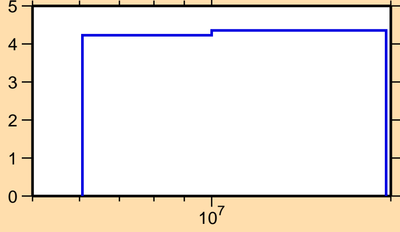
\Delta\sigma/\sigma vs. E for ^{56}\text{Cr}(n,el.)
