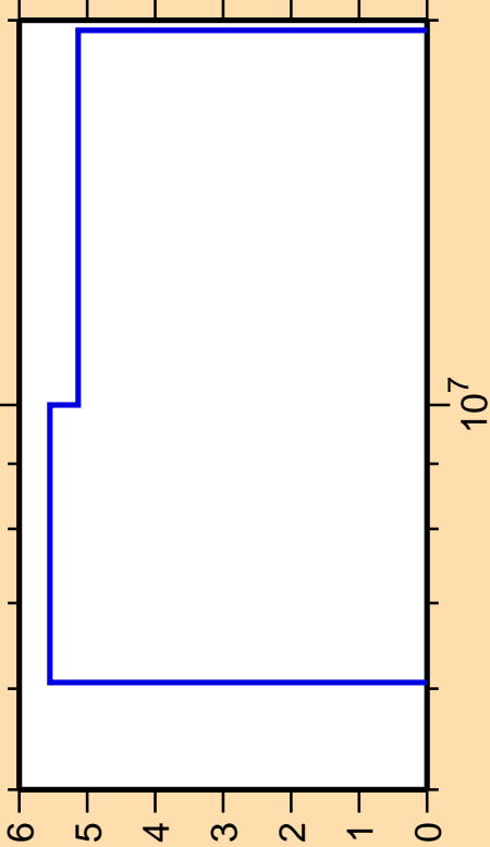
\Delta\sigma/\sigma vs. E for ^{56}\text{Cr}(n,2n)
