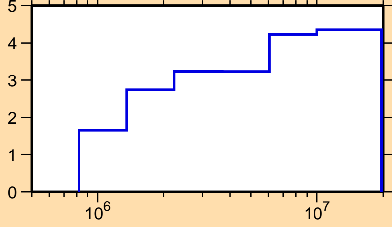
\Delta\sigma/\sigma vs. E for ^{56}\text{Cr}(n,\text{el.})
