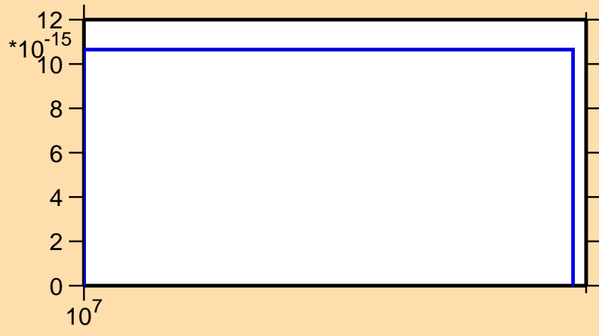
\sigma vs. E for ^{56}\text{Cr}(n,nt)
