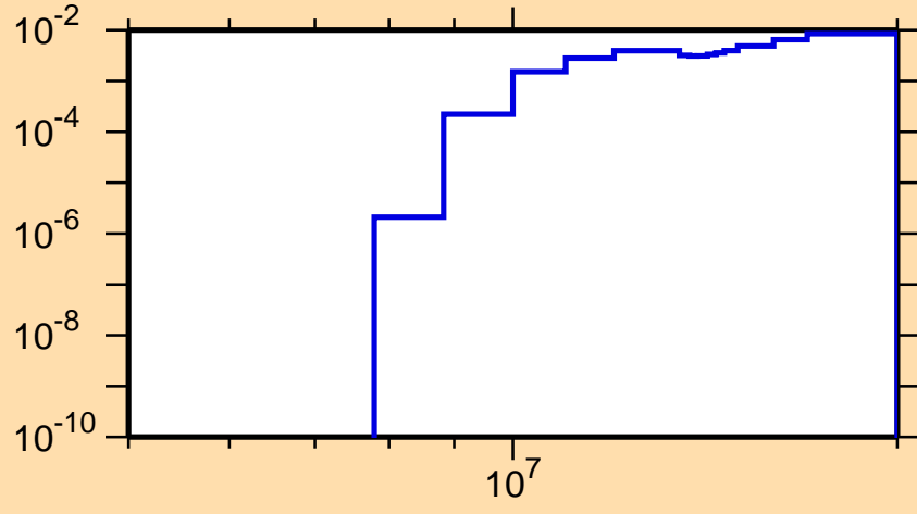
\sigma vs. E for ^{57}\text{Cr}(n,p)
