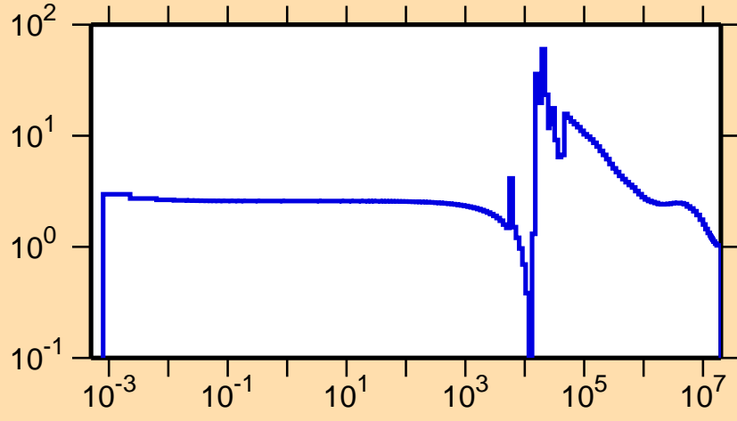
\sigma vs. E for ^{57}\text{Cr}(n,\text{el.})
