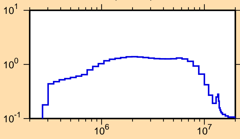
\sigma vs. E for ^{57}\text{Cr}(n,\text{inel.})
