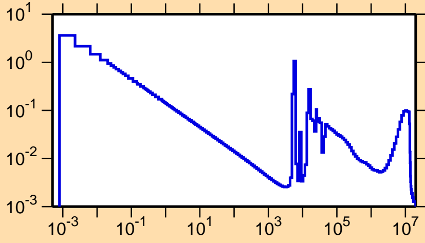
\sigma vs. E for ^{57}\text{Cr}(n,\gamma)
