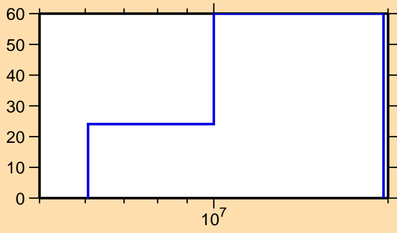
\Delta\sigma/\sigma vs. E for ^{57}\text{Cr}(n,n_1)
