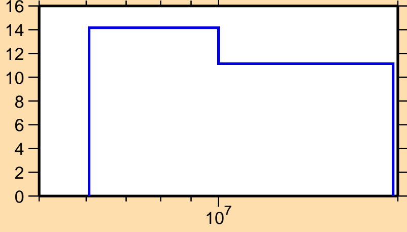
\Delta\sigma/\sigma vs. E for ^{57}\text{Cr}(n,el.)
