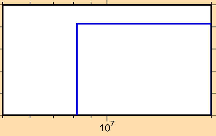
\sigma vs. E for ^{57}\text{Cr}(n,\text{nd})
