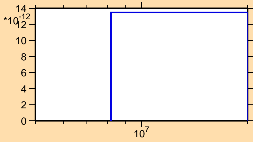
\sigma vs. E for ^{57}\text{Cr}(n,nt)
