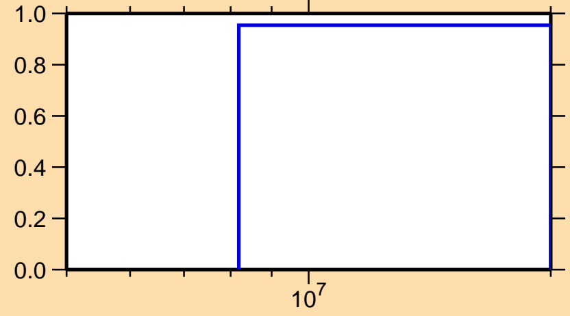
\sigma vs. E for ^{57}\text{Cr}(n,2n)
