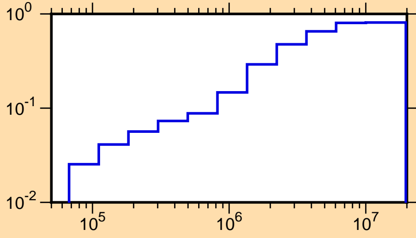
\mu vs. E for ^{58}\text{Cr}(\text{mt251})
