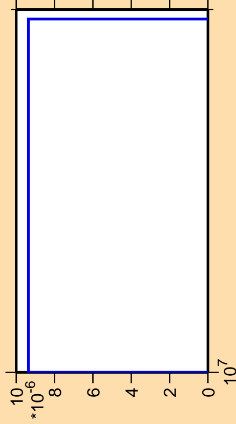
\Delta\sigma/\sigma vs. E for ^{58}\text{Cr}(n,\text{nd})
