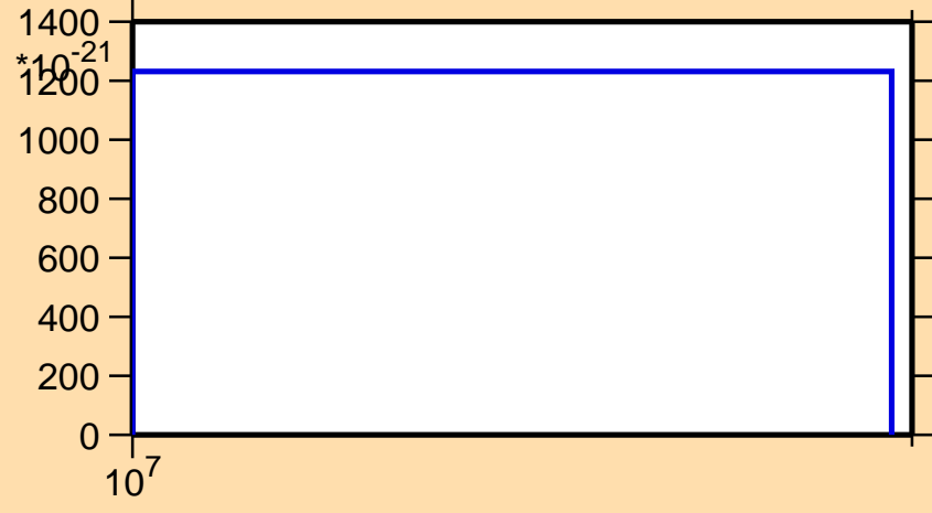
\sigma vs. E for ^{58}\text{Cr}(n,\text{nd})
