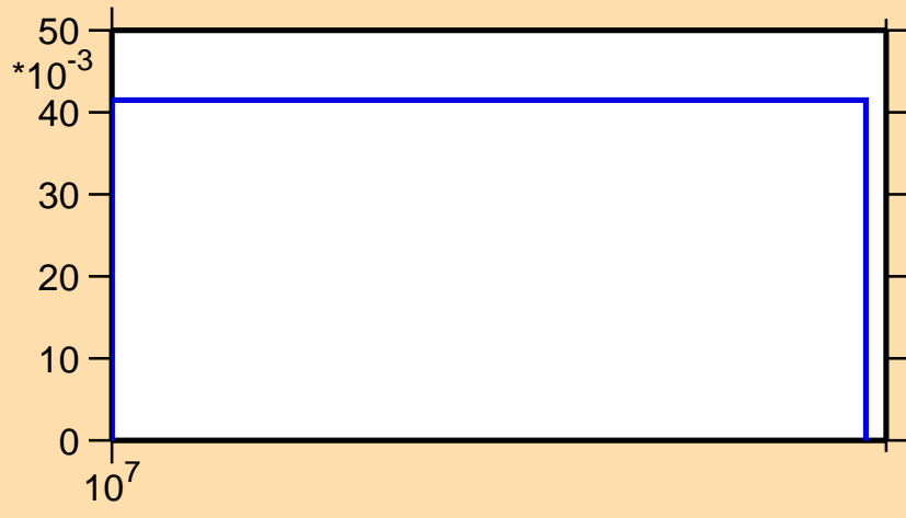
\sigma vs. E for ^{58}\text{Cr}(n,3n)
