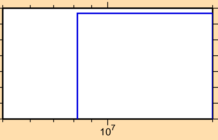
\sigma vs. E for ^{58}\text{Cr}(n,3n)
