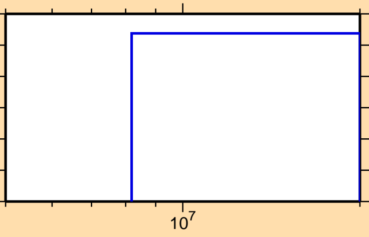
\sigma vs. E for ^{58}\text{Cr}(n,p)
