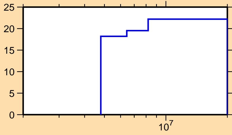
\Delta\sigma/\sigma vs. E for ^{58}\text{Cr}(n,n\text{onel.})
