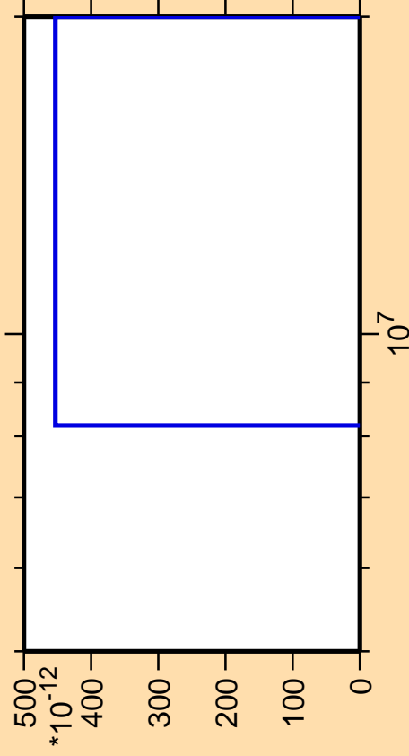
\Delta\sigma/\sigma vs. E for ^{58}\text{Cr}(n,\text{He}3)
