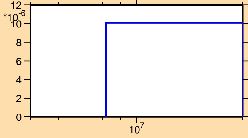
\sigma vs. E for ^{58}\text{Cr}(n,d)
