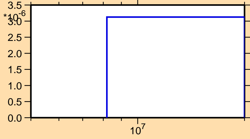
\sigma vs. E for ^{58}\text{Cr}(n,\alpha)
