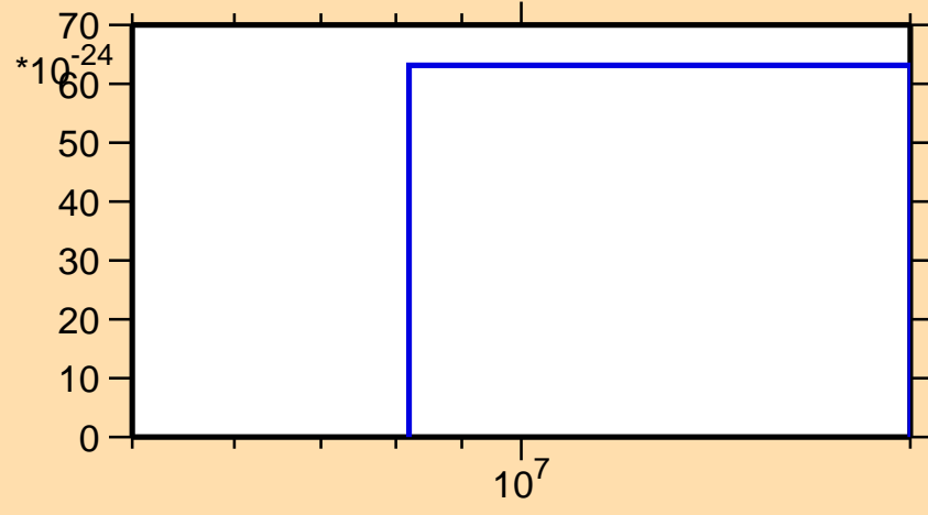
\sigma vs. E for ^{58}\text{Cr}(n,\text{He}3)
