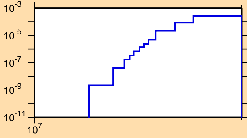
\sigma vs. E for ^{59}\text{Cr}(n,n\alpha)
