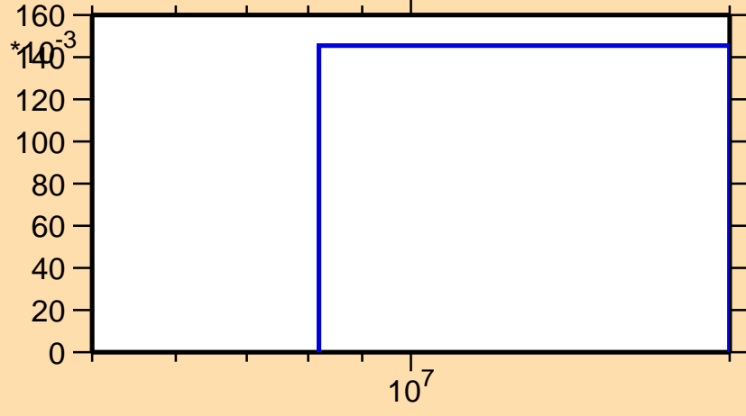
\sigma vs. E for ^{59}\text{Cr}(n,3n)
