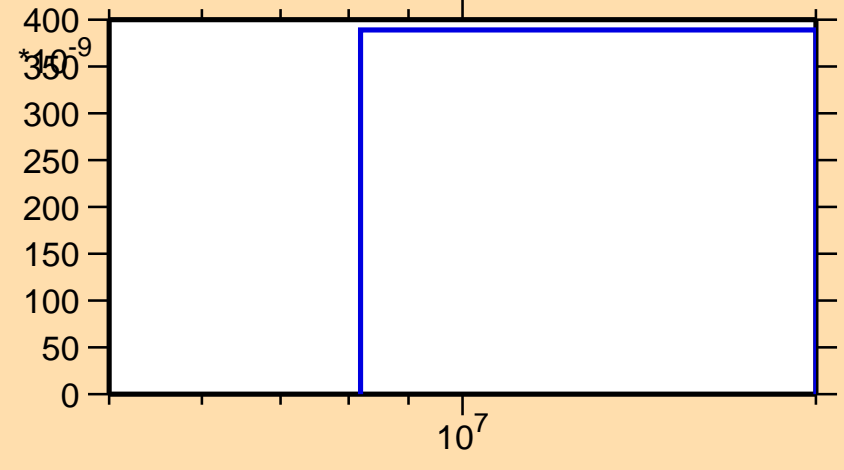
\sigma vs. E for ^{59}\text{Cr}(n,np)
