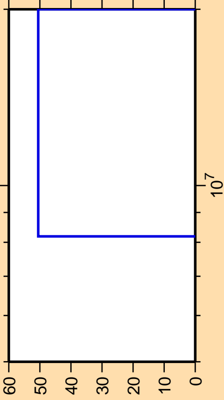
\Delta\sigma/\sigma vs. E for ^{59}\text{Cr}(n,p)
