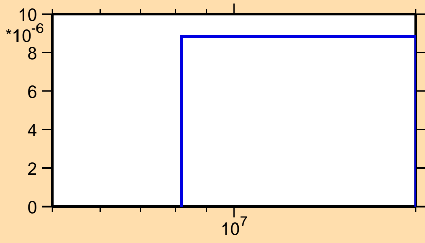
\sigma vs. E for ^{59}\text{Cr}(n,\alpha)
