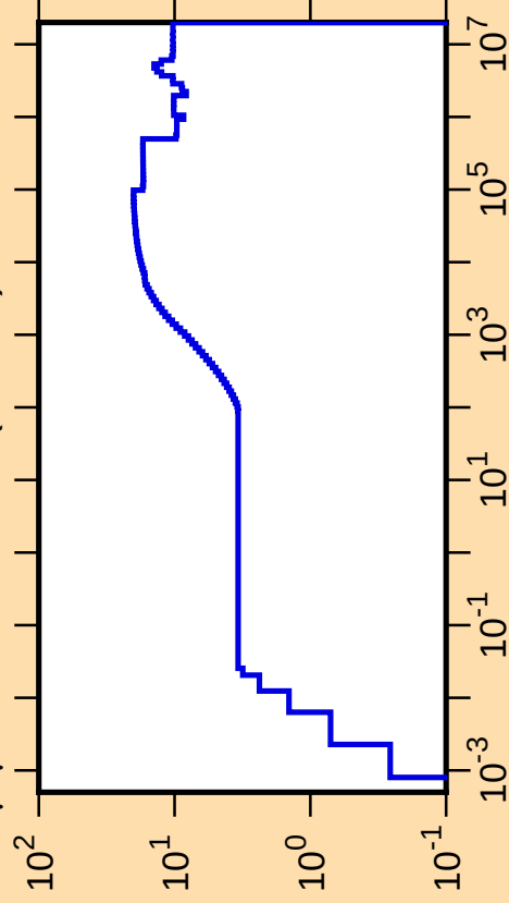
\Delta\mu/\mu vs. E for ^{115}\text{Cs}(\text{mt251})
