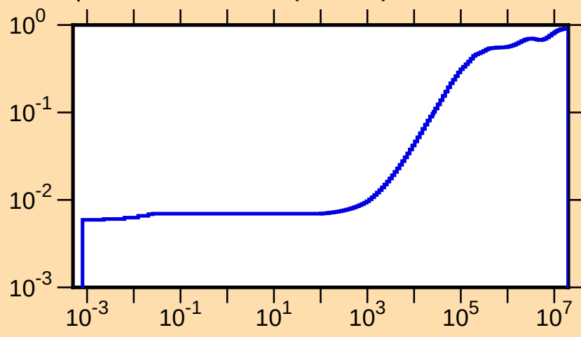
\mu vs. E for ^{115}\text{Cs}(\text{mt251})
