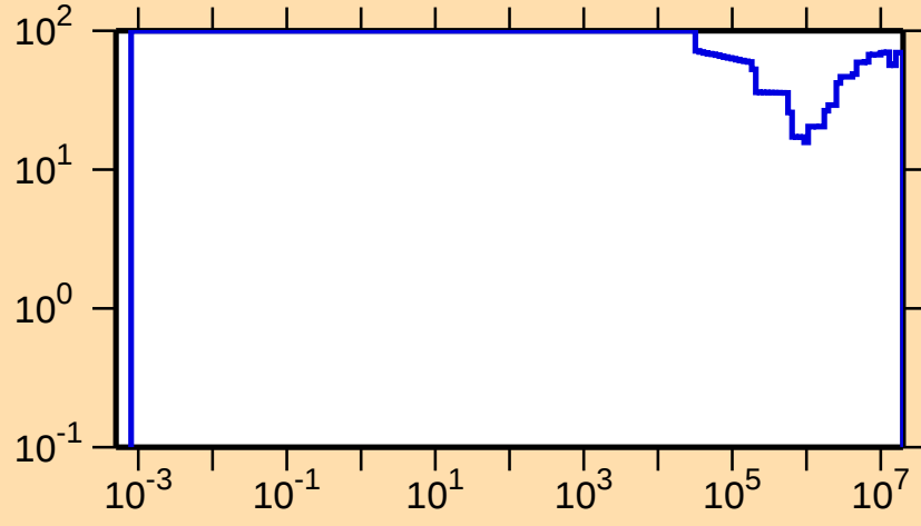
\Delta\sigma/\sigma vs. E for ^{117}\text{Cs}(n,p)
