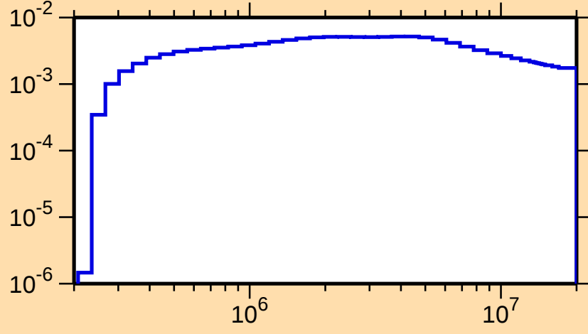
\sigma vs. E for ^{117}\text{Cs}(n,n_1)
