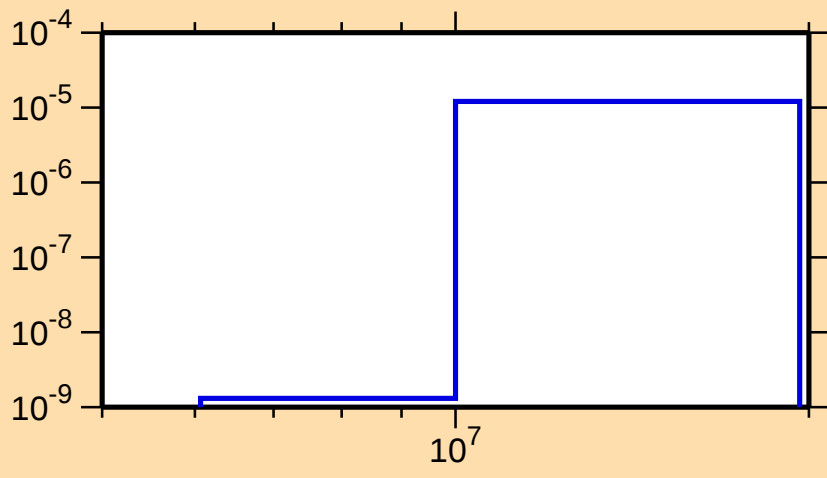
\sigma vs. E for ^{117}\text{Cs}(\text{mt117})
