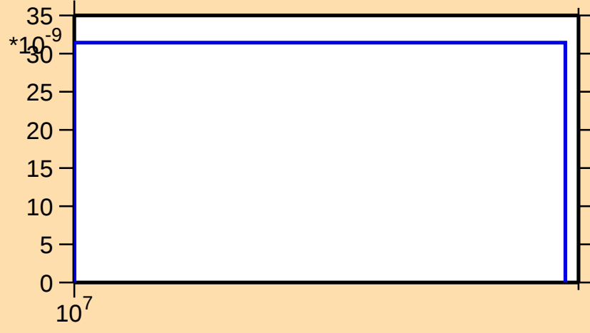
\sigma vs. E for ^{117}\text{Cs}(n,\text{nd})
