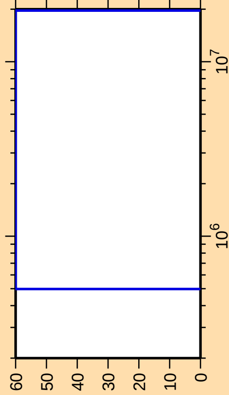
\Delta\sigma/\sigma vs. E for ^{117}\text{Cs}(n,\alpha)
