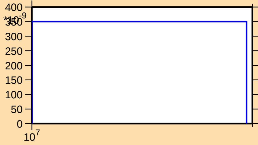
\sigma vs. E for ^{117}\text{Cs}(n,\text{pt})
