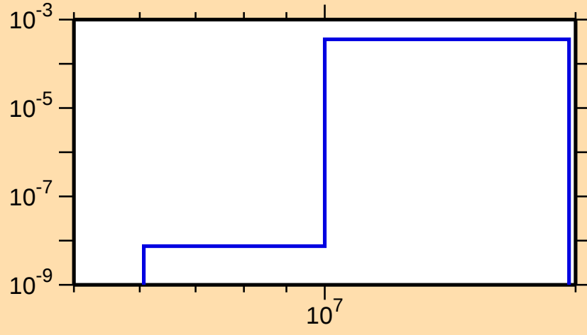
\sigma vs. E for ^{117}\text{Cs} (mt 45)
