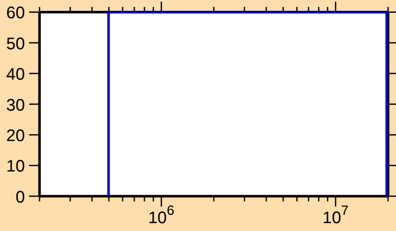
\Delta\sigma/\sigma vs. E for ^{117}\text{Cs}(n,n\text{cont.})
