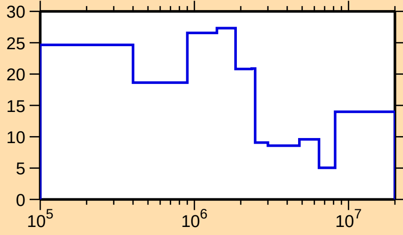
\Delta\sigma/\sigma vs. E for ^{117}\text{Cs}(n,\text{tot.})
