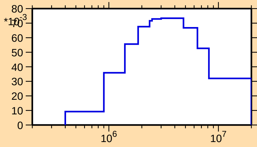
\sigma vs. E for ^{117}\text{Cs}(n,n_4)
