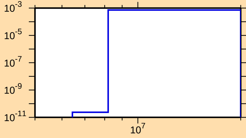
\sigma vs. E for ^{117}\text{Cs}(n,\text{pd})
