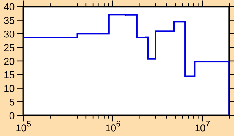
\Delta\sigma/\sigma vs. E for ^{117}\text{Cs}(n,\text{el.})
