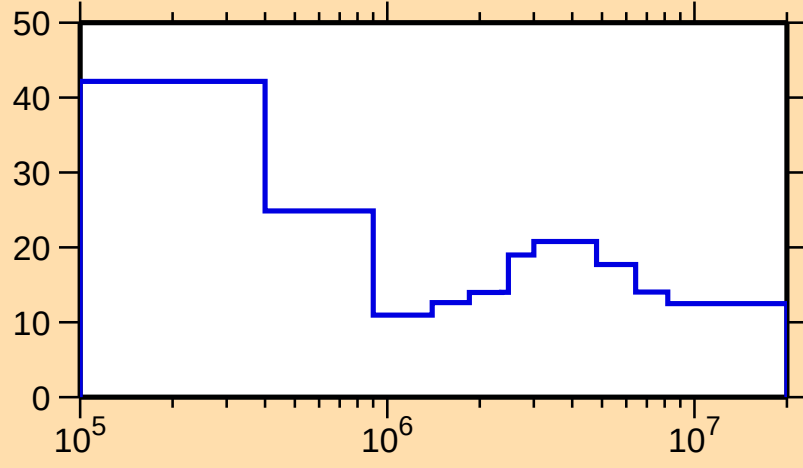
\Delta\sigma/\sigma vs. E for ^{117}\text{Cs}(n,\text{nonel.})
