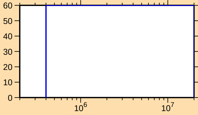
\Delta\sigma/\sigma vs. E for ^{117}\text{Cs}(n,n\text{cont.})
