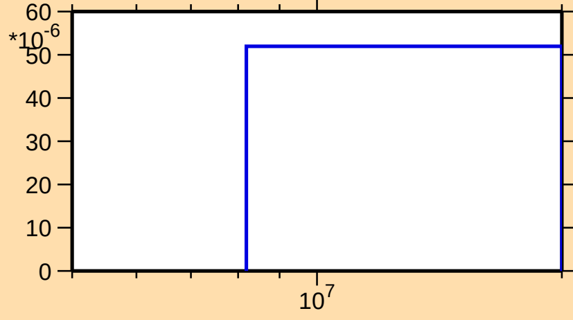
\sigma vs. E for ^{119}\text{Cs}(n,\text{pd})
