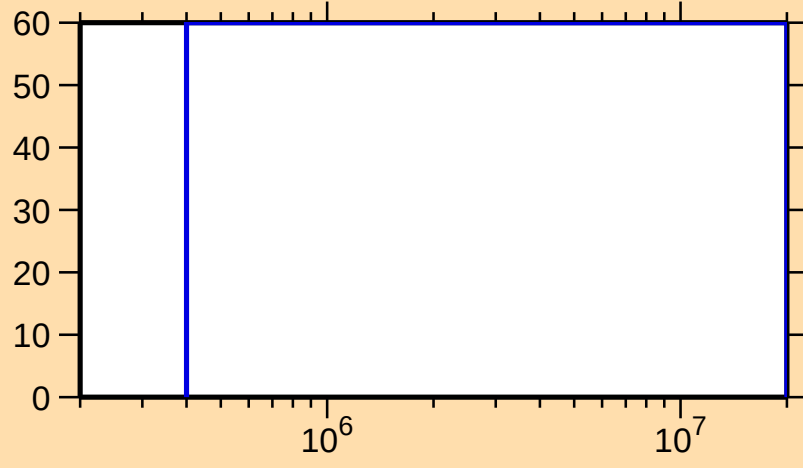
\Delta\sigma/\sigma vs. E for ^{119}\text{Cs}(n,n\text{cont.})
