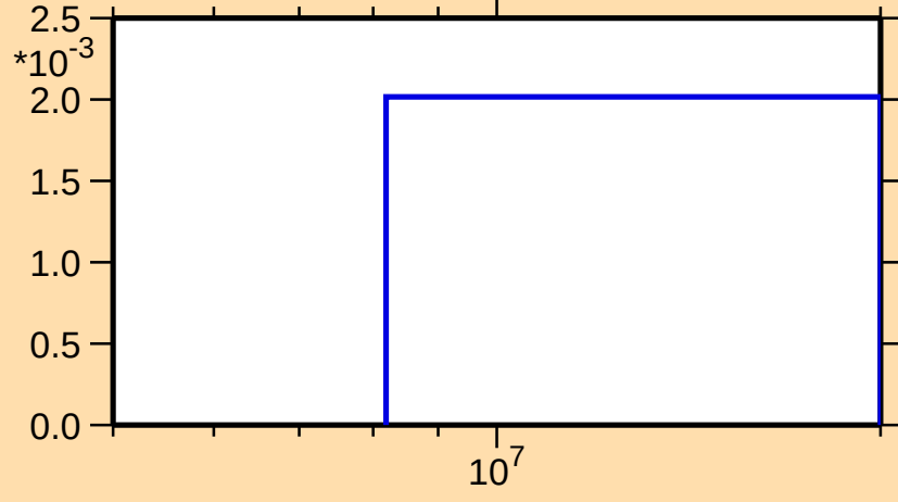
\sigma vs. E for ^{119}\text{Cs}(n,2n)
