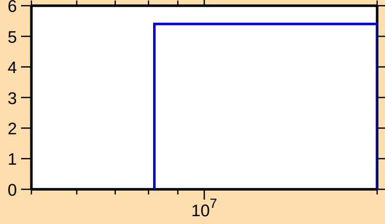
\Delta\sigma/\sigma vs. E for ^{119}\text{Cs}(n,\text{nonel.})
