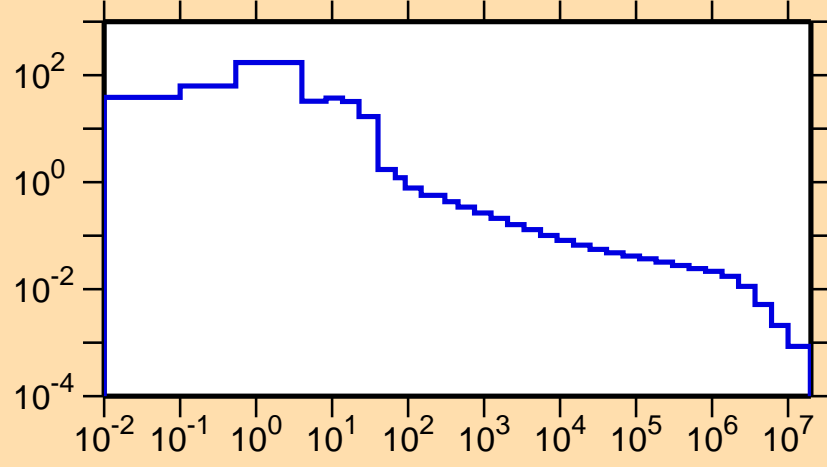
\sigma vs. E for ^{119}\text{Cs}(n,\gamma)
