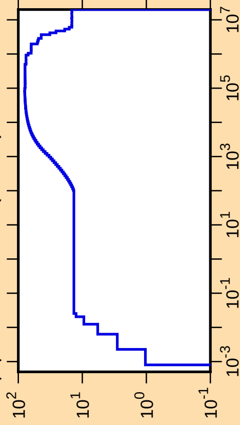
\Delta\mu/\mu vs. E for ^{120}\text{Cs}(\text{mt251})
