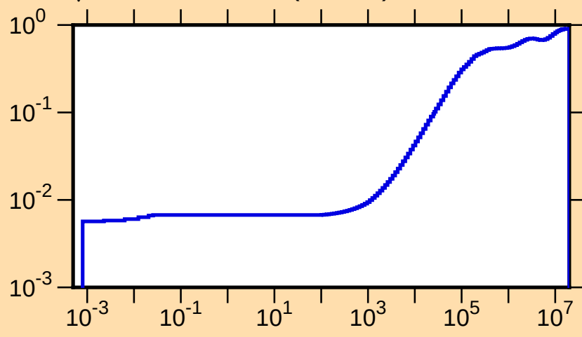
\mu vs. E for ^{120}\text{Cs}(\text{mt251})
