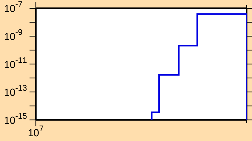
\sigma vs. E for ^{121}\text{Cs}(n,2n\alpha)
