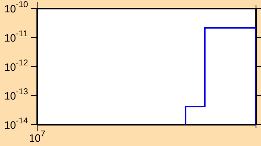
\sigma vs. E for ^{121}\text{Cs} (mt 34)
