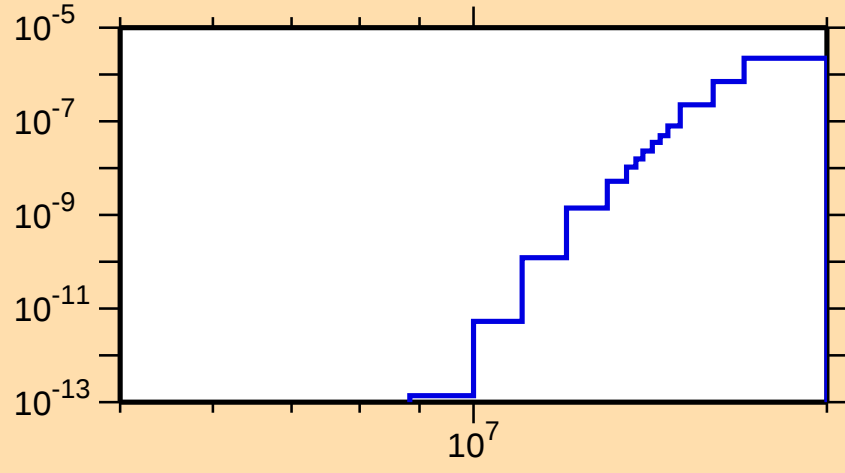
\sigma vs. E for ^{121}\text{Cs}(\text{mt117})
