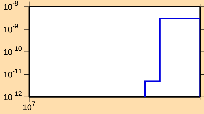
\sigma vs. E for ^{121}\text{Cs}(n,\text{pt})
