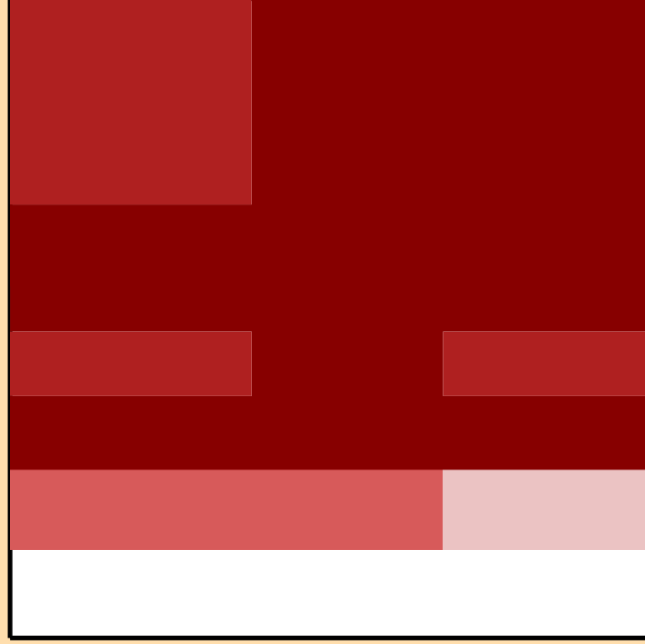
\Delta\sigma/\sigma vs. E for ^{121}\text{Cs}(n,\text{tot.})
