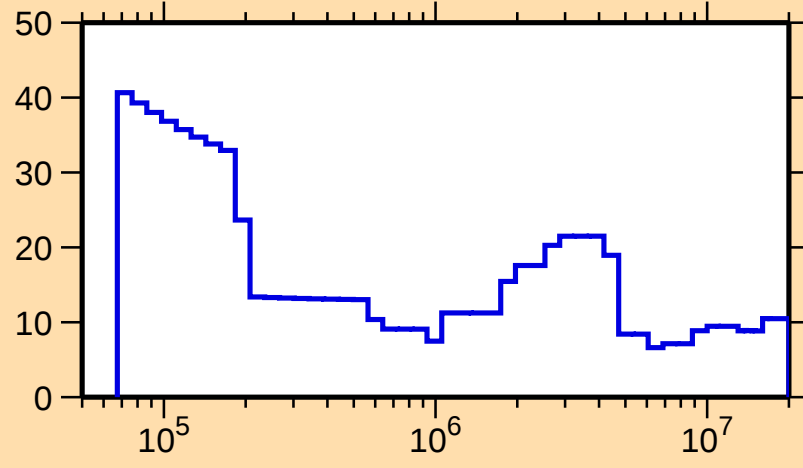
\Delta\sigma/\sigma vs. E for ^{121}\text{Cs}(n,\text{el.})
