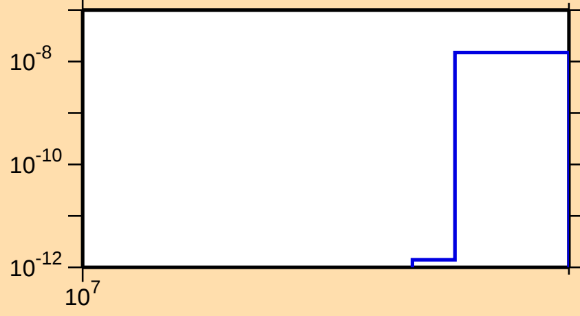
\sigma vs. E for ^{121}\text{Cs}(n,nt)
