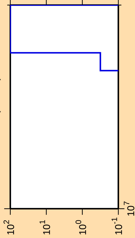
\Delta\sigma/\sigma vs. E for ^{121}\text{Cs} (mt 34)
