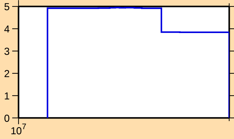
\Delta\sigma/\sigma vs. E for ^{121}\text{Cs}(n,\text{nonel.})
