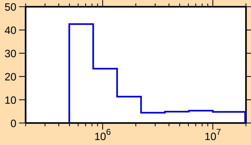
\Delta\sigma/\sigma vs. E for ^{121}\text{Cs}(n,\text{nonel.})
