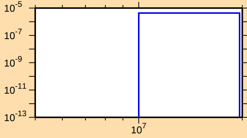
\sigma vs. E for ^{121}\text{Cs}(n,\text{pd})
