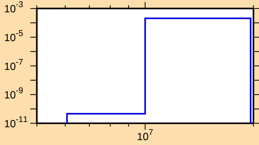
\sigma vs. E for ^{121}\text{Cs}(n,t)
