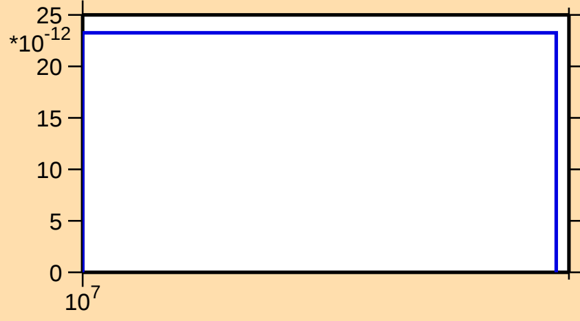
\sigma vs. E for ^{121}\text{Cs}(n,\text{pt})
