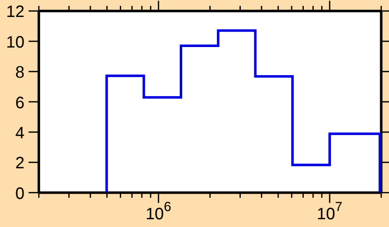
\Delta\sigma/\sigma vs. E for ^{121}\text{Cs}(n,\text{tot.})
