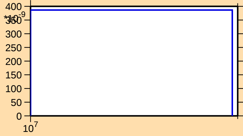
\sigma vs. E for ^{121}\text{Cs}(n,\text{nd})
