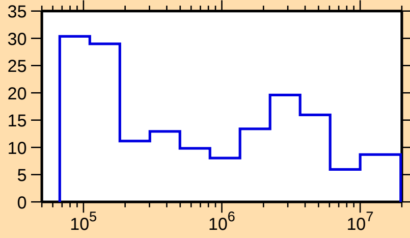
\Delta\sigma/\sigma vs. E for ^{121}\text{Cs}(n,\text{el.})
