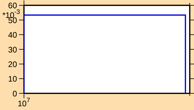
\sigma vs. E for ^{121}\text{Cs}(n,2n)
