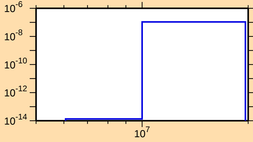
\sigma vs. E for ^{121}\text{Cs}(\text{mt117})
