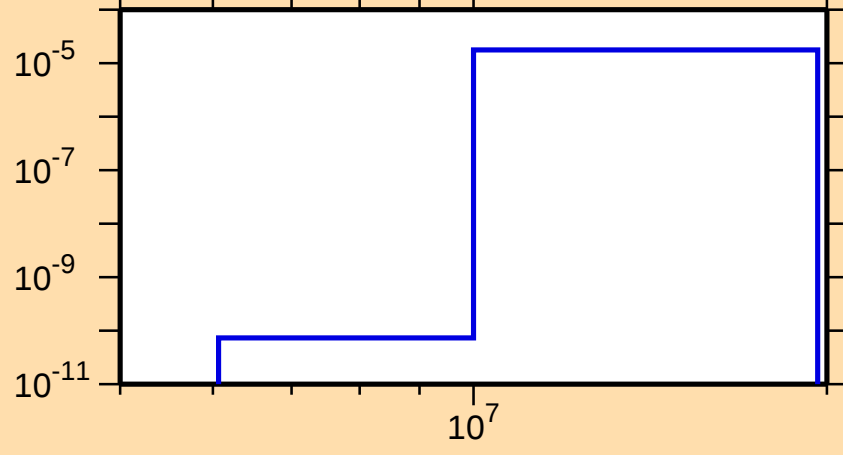
\sigma vs. E for ^{121}\text{Cs}(n,\text{He}3)
