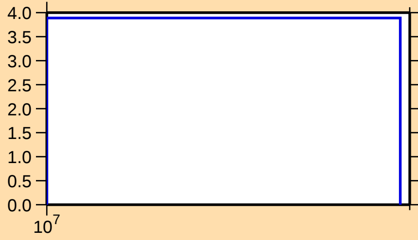
\Delta\sigma/\sigma vs. E for ^{121}\text{Cs}(n,\text{tot.})
