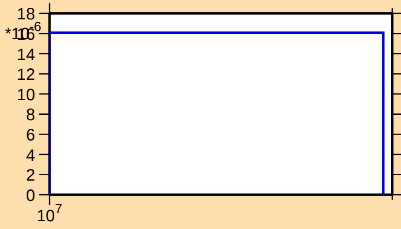
\sigma vs. E for ^{121}\text{Cs}(n,2np)
