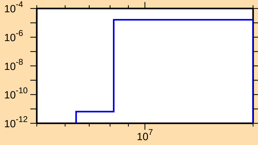
\sigma vs. E for ^{121}\text{Cs}(n,\text{He}3)
