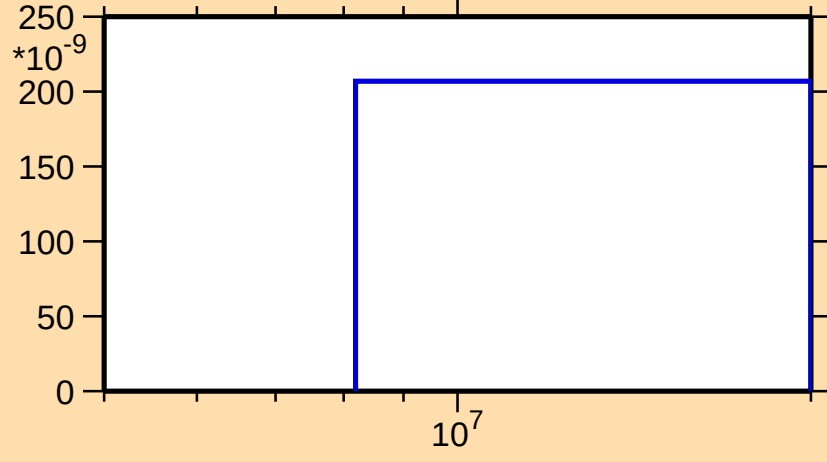
\sigma vs. E for ^{121}\text{Cs}(n,\text{nd})
