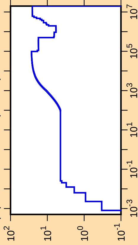
\Delta\mu/\mu vs. E for ^{122}\text{Cs}(\text{mt251})
