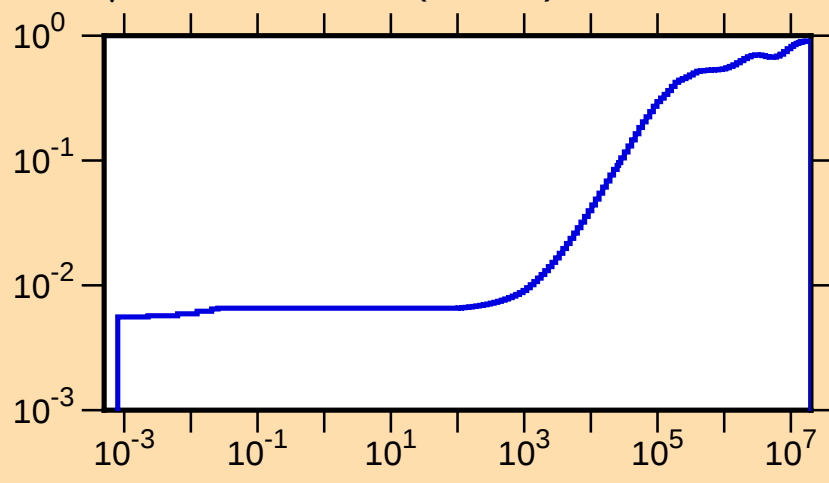
\mu vs. E for ^{122}\text{Cs}(\text{mt251})
