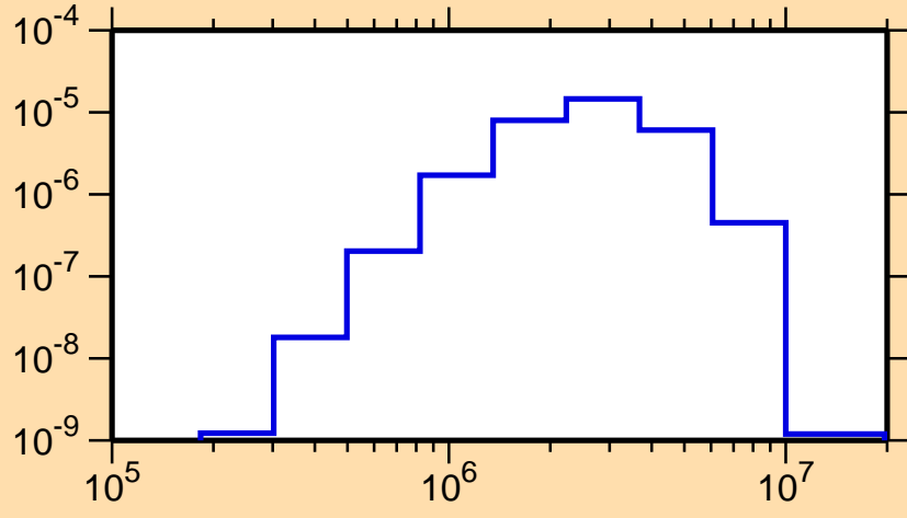
\sigma vs. E for ^{122}\text{Cs}(n,n_4)
