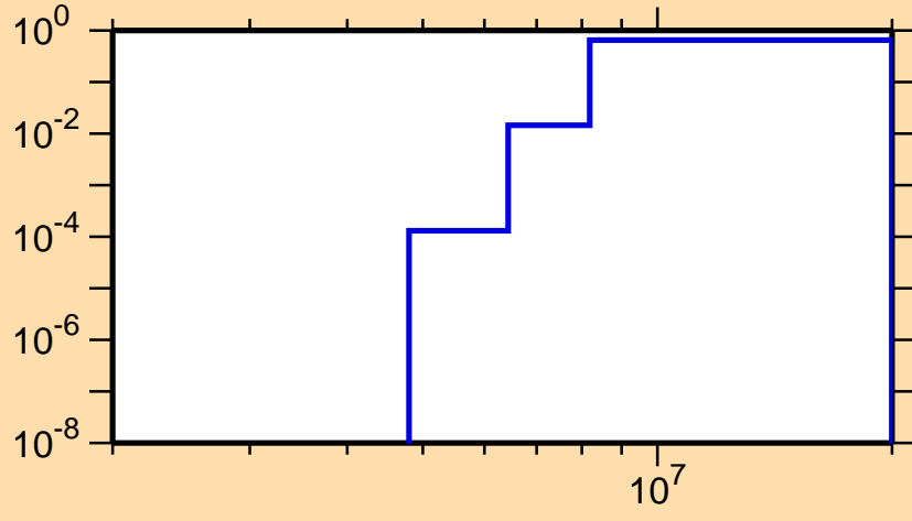
\sigma vs. E for ^{122}\text{Cs}(n,np)
