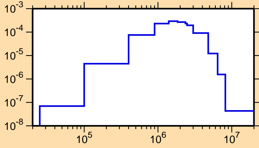
\sigma vs. E for ^{122}\text{Cs}(n,n_3)
