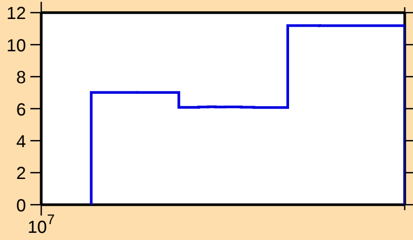
\Delta\sigma/\sigma vs. E for ^{123}\text{Cs}(n,\text{el.})
