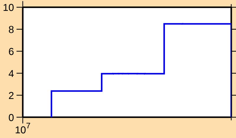
\Delta\sigma/\sigma vs. E for ^{123}\text{Cs}(n,\text{tot.})
