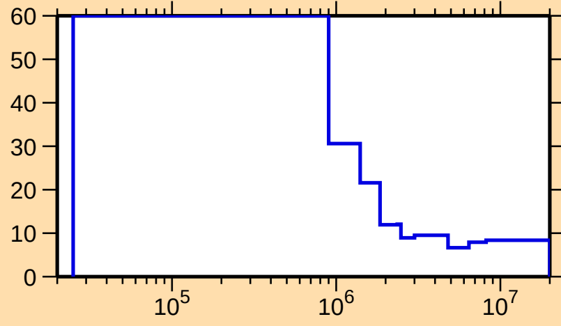
\Delta\sigma/\sigma vs. E for ^{123}\text{Cs}(n,\text{nonel.})
