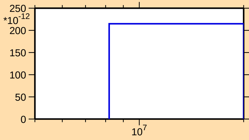
\sigma vs. E for ^{123}\text{Cs}(n,nt)
