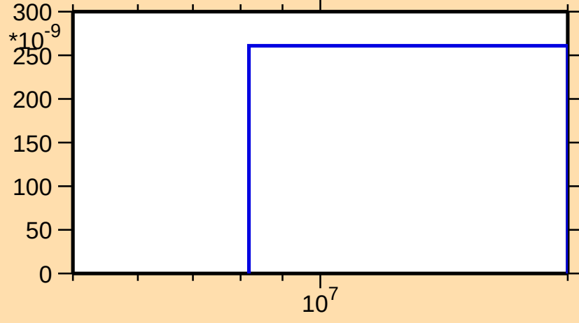
\sigma vs. E for ^{123}\text{Cs}(n,nd)
