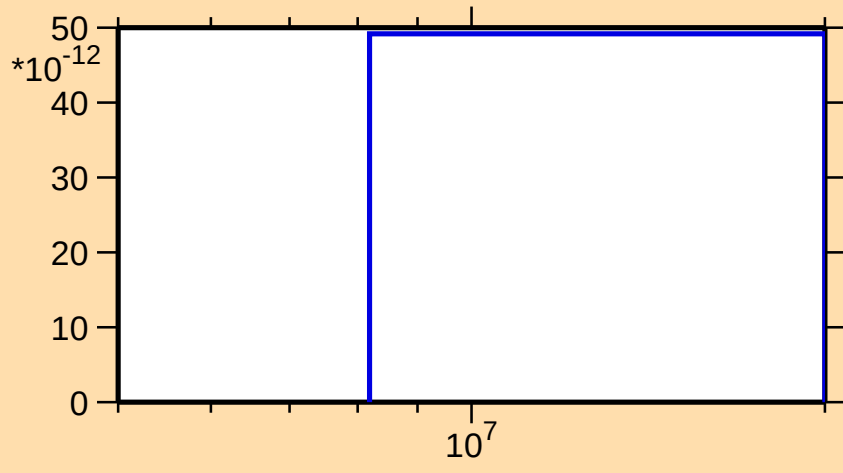
\sigma vs. E for ^{123}\text{Cs}(n,2n\alpha)
