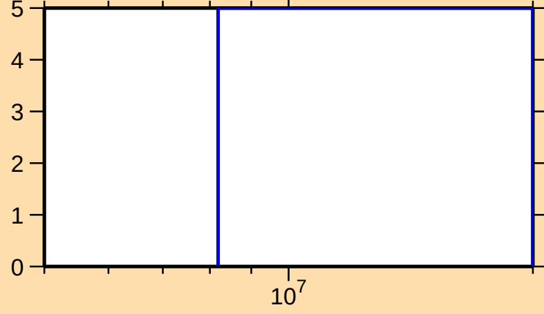
\Delta\sigma/\sigma vs. E for ^{123}\text{Cs}(n,\text{el.})
