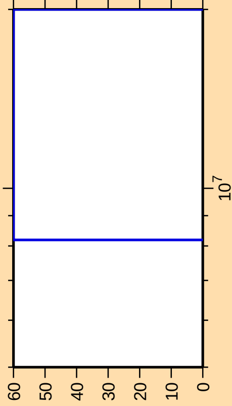
\Delta\sigma/\sigma vs. E for ^{123}\text{Cs}(n,nd)
