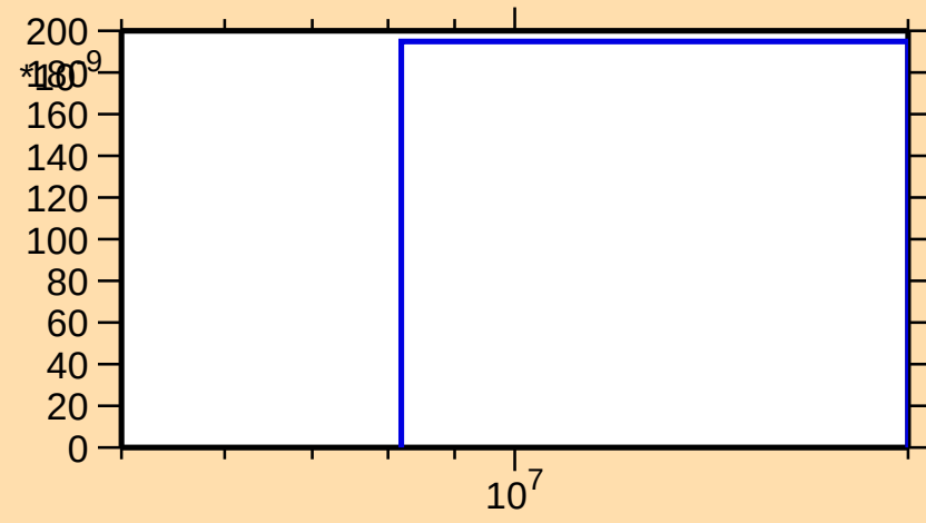
\sigma vs. E for ^{123}\text{Cs} (mt 45)
