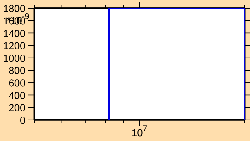
\sigma vs. E for ^{123}\text{Cs}(n,\text{He}3)
