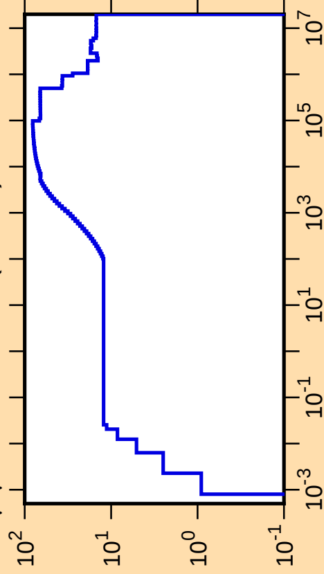
\Delta\mu/\mu vs. E for ^{124}\text{Cs}(\text{mt251})
