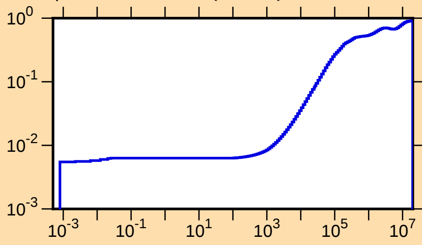
\mu vs. E for ^{124}\text{Cs}(\text{mt251})
