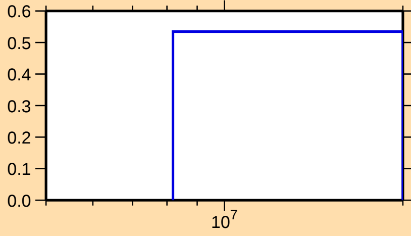
\sigma vs. E for ^{124}\text{Cs}(n,2n)
