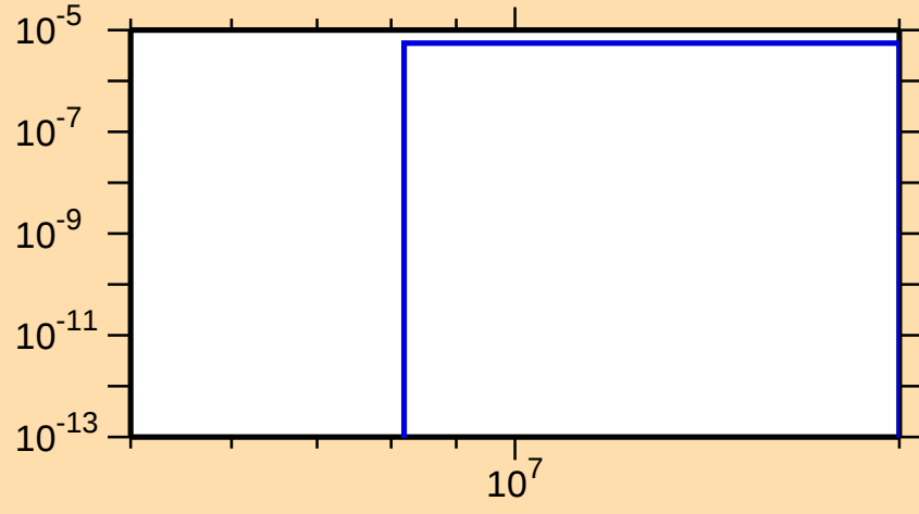
\sigma vs. E for ^{124}\text{Cs}(n,\text{He}3)
