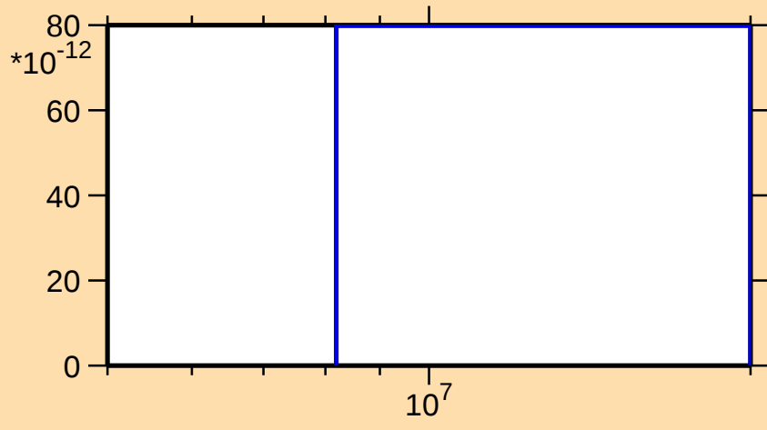
\sigma vs. E for ^{124}\text{Cs}(\text{mt117})
