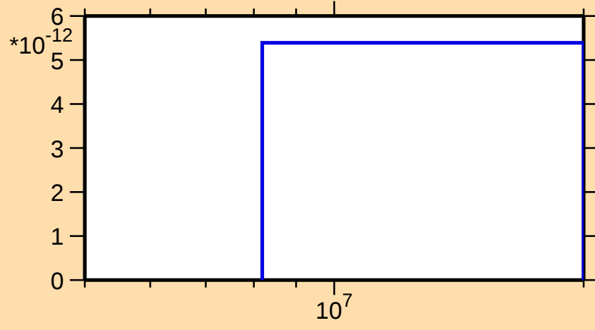
\sigma vs. E for ^{124}\text{Cs}(\text{mt } 34)
