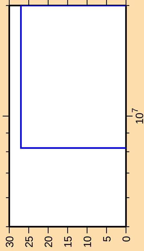
\Delta\sigma/\sigma vs. E for ^{124}\text{Cs}(\text{mt } 34)
