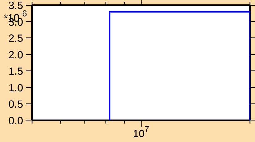
\sigma vs. E for ^{124}\text{Cs}(n,\text{nd})
