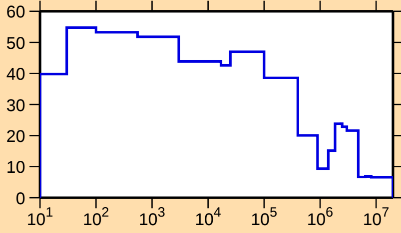
\Delta\sigma/\sigma vs. E for ^{124}\text{Cs}(n,\text{el.})
