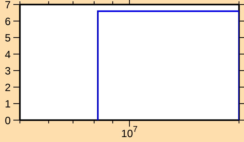
\Delta\sigma/\sigma vs. E for ^{124}\text{Cs}(n,\text{el.})
