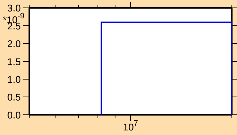
\sigma vs. E for ^{124}\text{Cs}(n,\text{pd})
