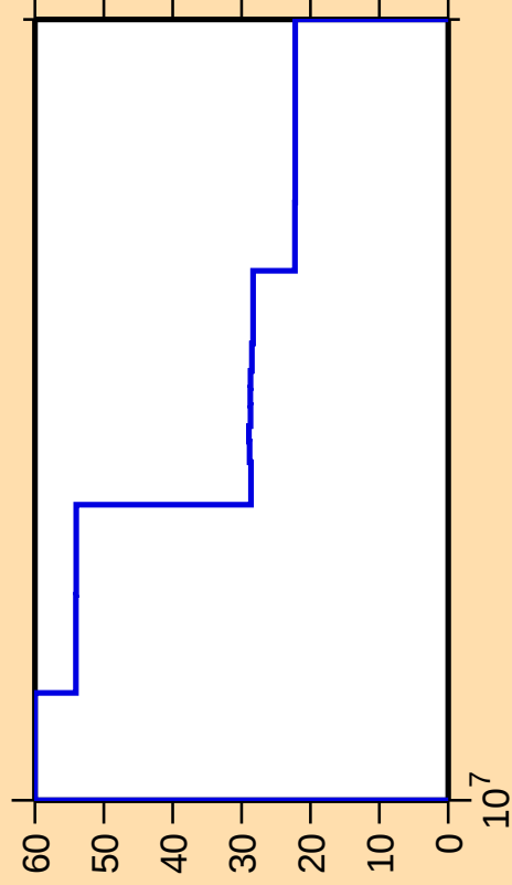
\Delta\sigma/\sigma vs. E for ^{125}\text{Cs}(n,2n)
