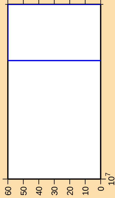
\Delta\sigma/\sigma vs. E for ^{125}\text{Cs}(n,\text{nt})
