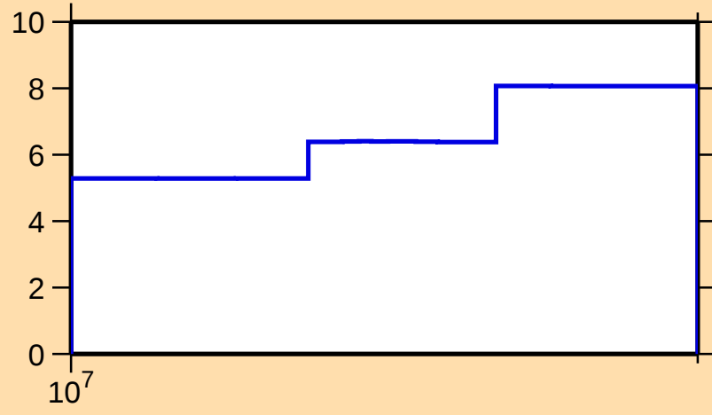
\Delta\sigma/\sigma vs. E for ^{125}\text{Cs}(n,\text{tot.})
