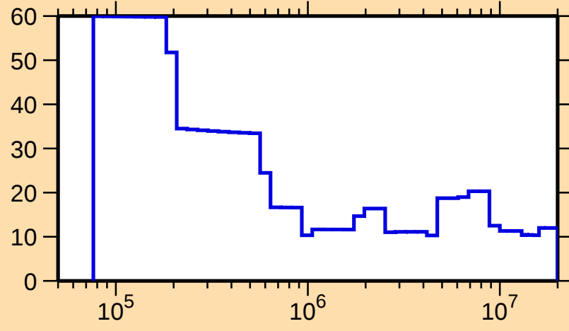
\Delta\sigma/\sigma vs. E for ^{125}\text{Cs}(n,\text{el.})
