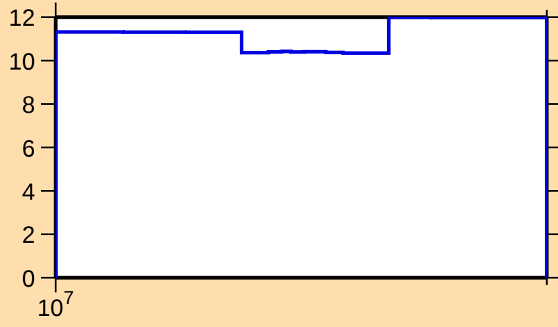
\Delta\sigma/\sigma vs. E for ^{125}\text{Cs}(n,\text{el.})
