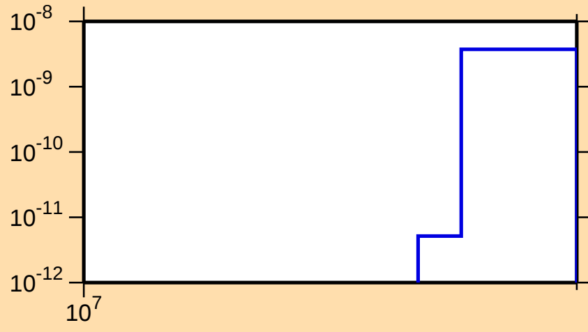
\sigma vs. E for ^{125}\text{Cs}(n,2n\alpha)
