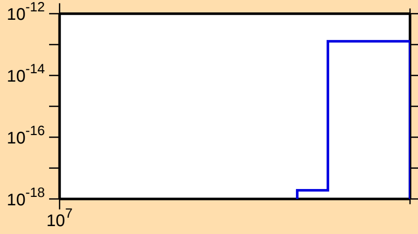
\sigma vs. E for ^{125}\text{Cs} (mt 34)
