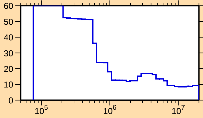
\Delta\sigma/\sigma vs. E for ^{125}\text{Cs}(n,\text{nonel.})
