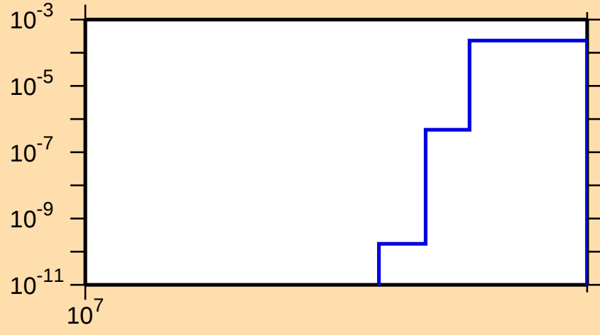
\sigma vs. E for ^{125}\text{Cs}(n,2np)
