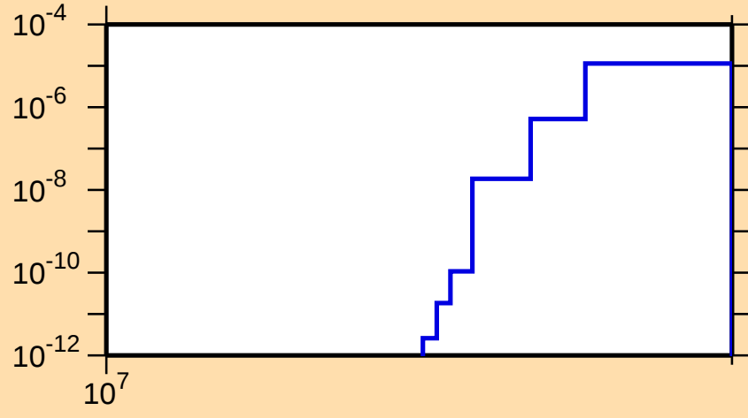
\sigma vs. E for ^{125}\text{Cs}(n,\text{nd})
