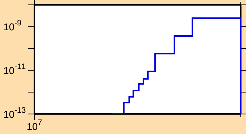
\sigma vs. E for ^{125}\text{Cs}(\text{mt117})
