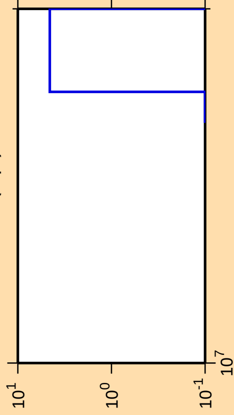
\Delta\sigma/\sigma vs. E for ^{125}\text{Cs}(n,\text{pt})
