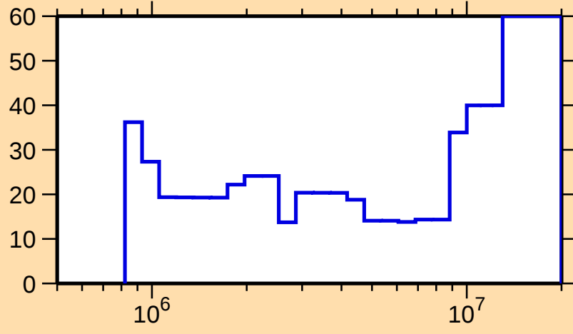
\Delta\sigma/\sigma vs. E for ^{125}\text{Cs}(n,\text{inel.})
