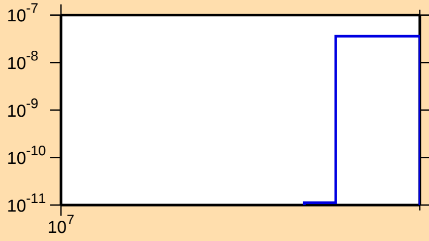
\sigma vs. E for ^{125}\text{Cs}(n,\text{nt})
