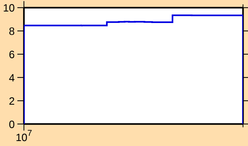
\Delta\sigma/\sigma vs. E for ^{125}\text{Cs}(n,\text{nonel.})
