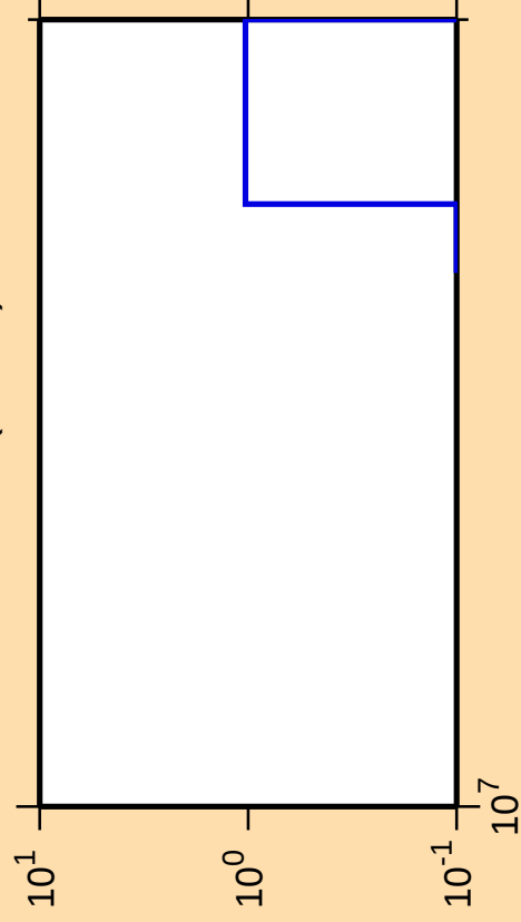
\Delta\sigma/\sigma vs. E for ^{125}\text{Cs} (mt 34)
