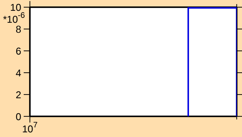
\sigma vs. E for ^{125}\text{Cs}(n,3n)
