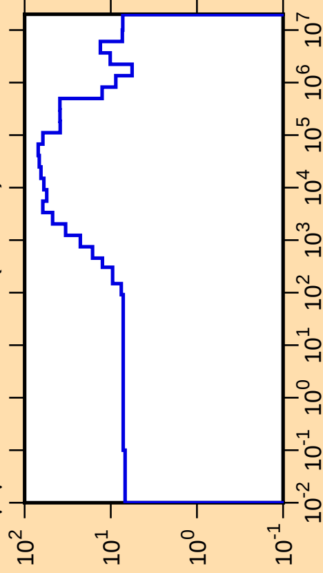
\Delta\mu/\mu vs. E for ^{125}\text{Cs}(\text{mt251})
