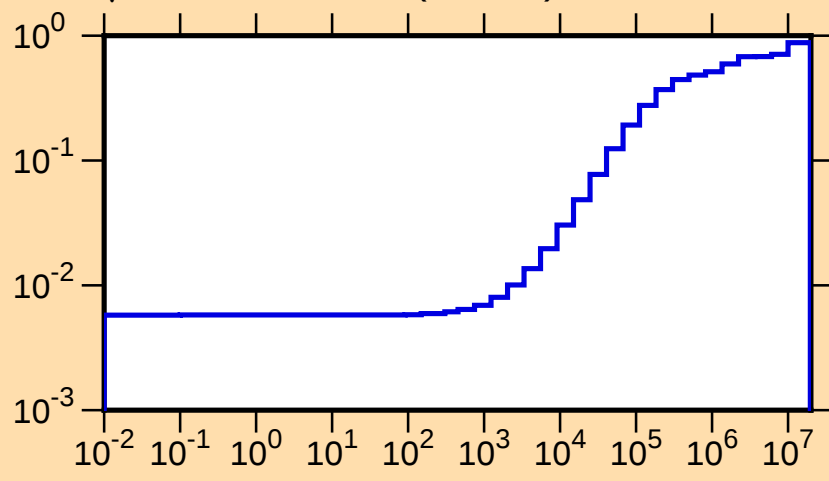
\mu vs. E for ^{125}\text{Cs}(\text{mt251})
