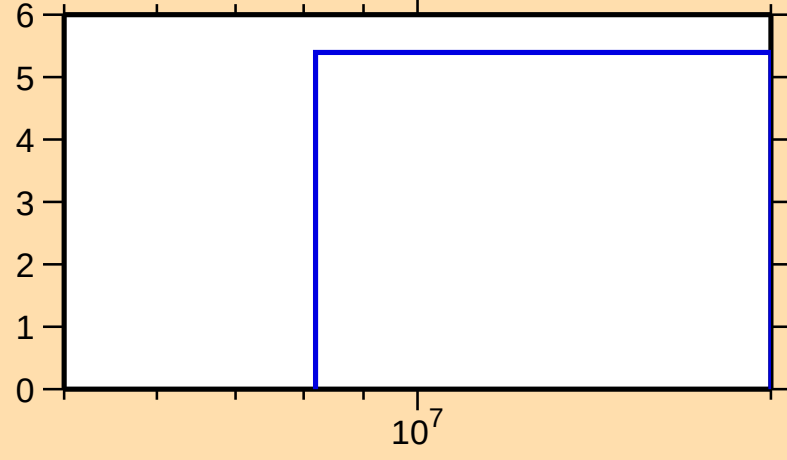
\Delta\sigma/\sigma vs. E for ^{125}\text{Cs}(n,\text{tot.})
