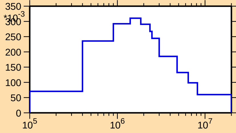
\sigma vs. E for ^{125}\text{Cs}(n,n_4)
