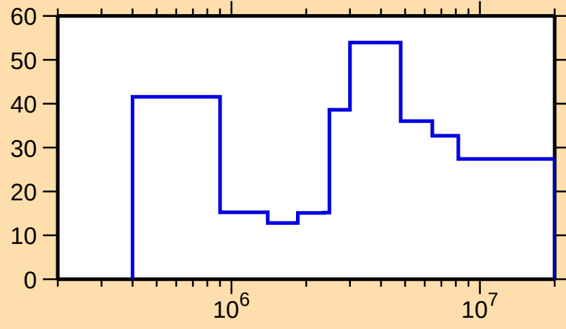
\Delta\sigma/\sigma vs. E for ^{125}\text{Cs}(n,n_1)
