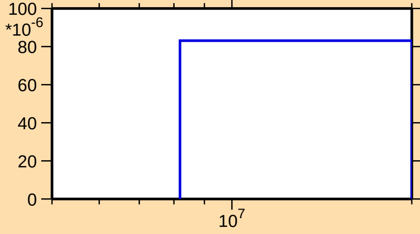
\sigma vs. E for ^{125}\text{Cs}(n,t)
