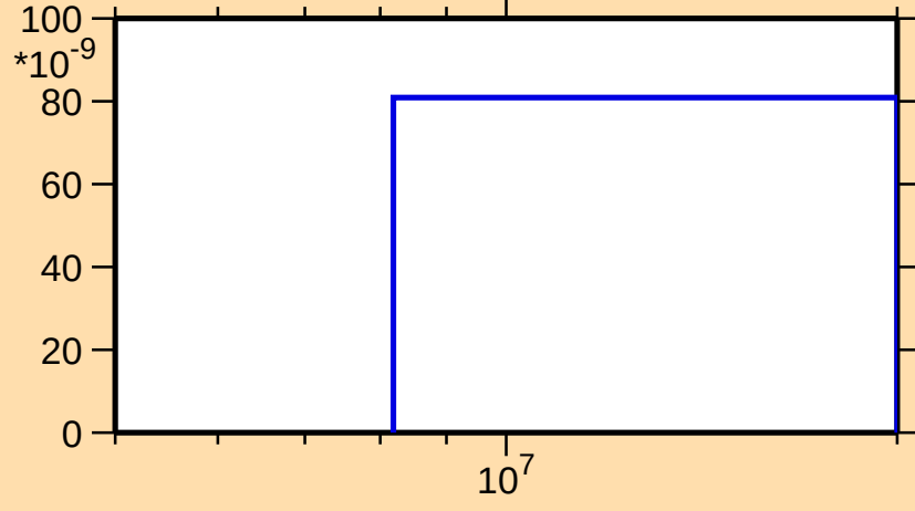
\sigma vs. E for ^{125}\text{Cs}(n,3n)
