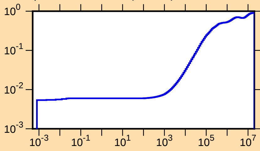
\mu vs. E for ^{126}\text{Cs}(\text{mt251})
