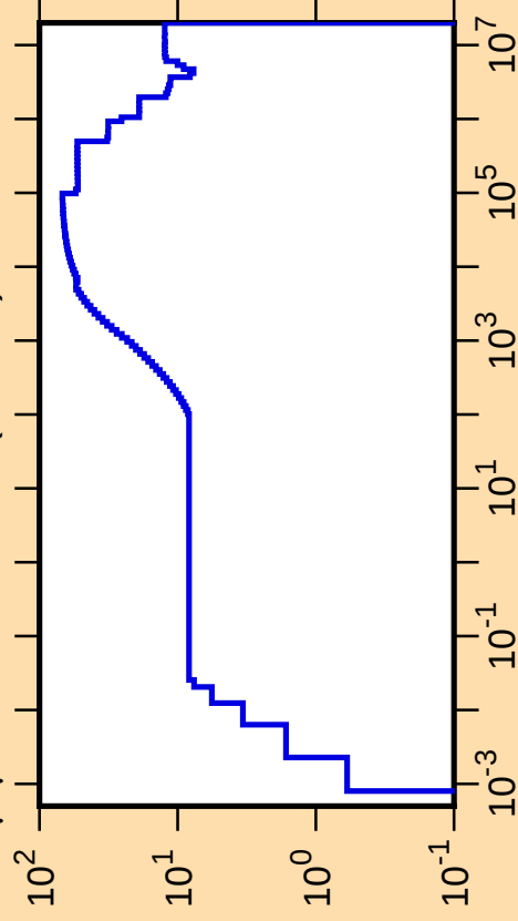
\Delta\mu/\mu vs. E for ^{126}\text{Cs}(\text{mt251})
