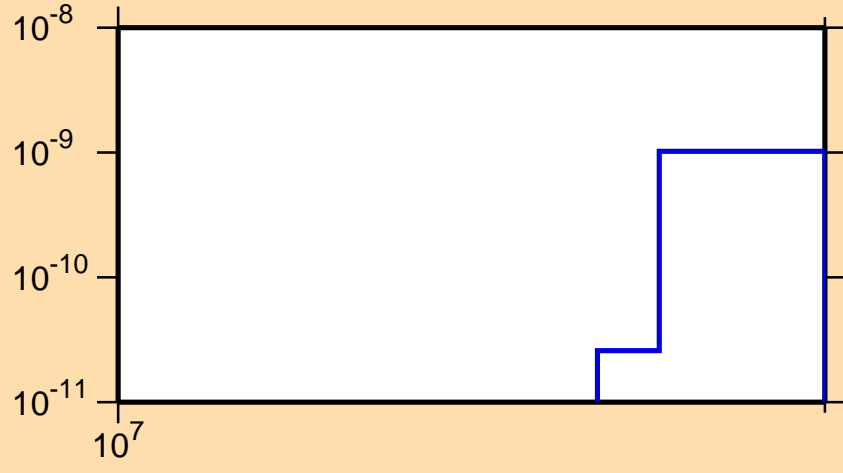
\sigma vs. E for ^{127}\text{Cs} (mt 45)
