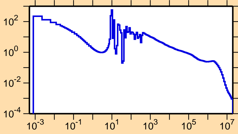
\sigma vs. E for ^{127}\text{Cs}(n,\gamma)
