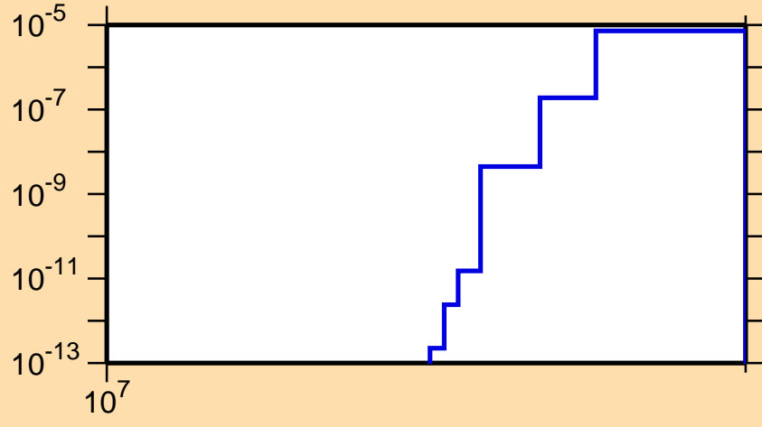
\sigma vs. E for ^{127}\text{Cs}(n,nd)
