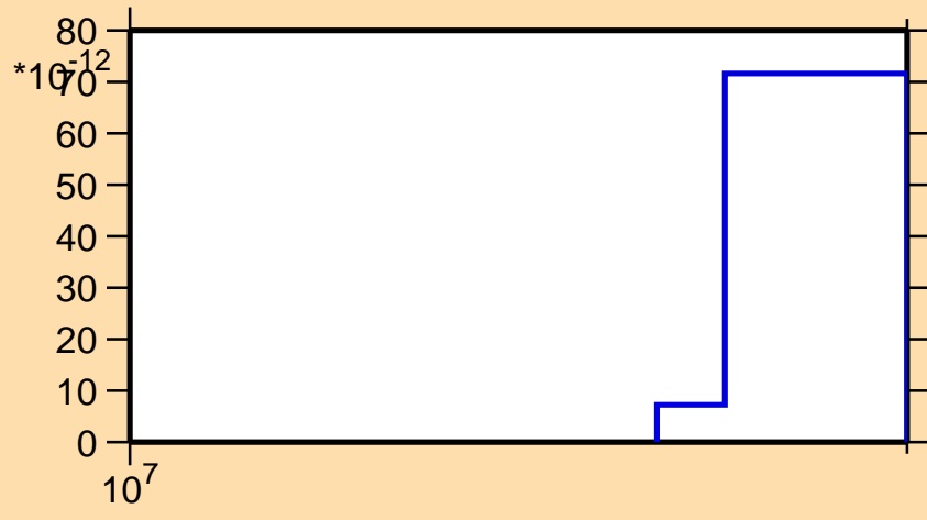
\sigma vs. E for ^{127}\text{Cs}(\text{mt117})
