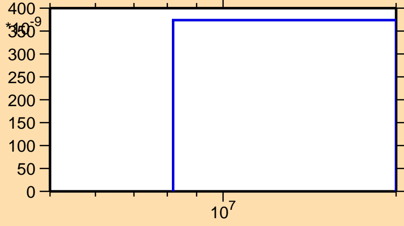
\sigma vs. E for ^{127}\text{Cs}(n,2np)
