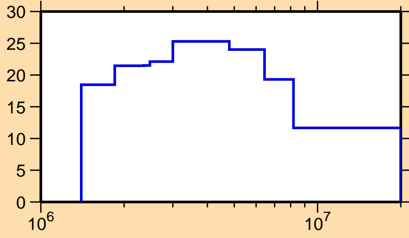
\Delta\sigma/\sigma vs. E for ^{127}\text{Cs}(n, el.)
