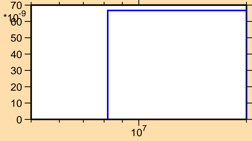
\sigma vs. E for ^{127}\text{Cs}(n,nd)
