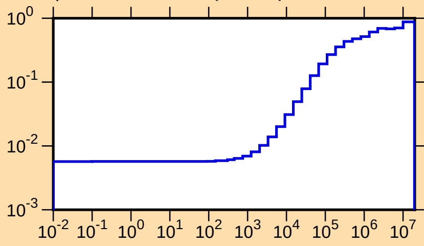
\mu vs. E for ^{128}\text{Cs}(\text{mt251})
