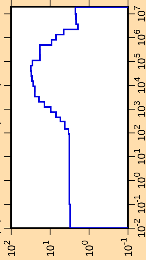
\Delta\mu/\mu vs. E for ^{128}\text{Cs}(\text{mt251})
