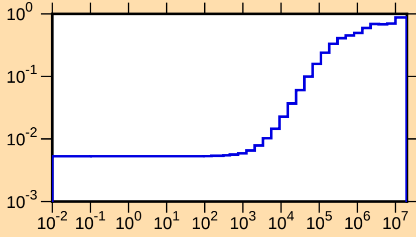
\mu vs. E for ^{131}\text{Cs}(\text{mt251})
