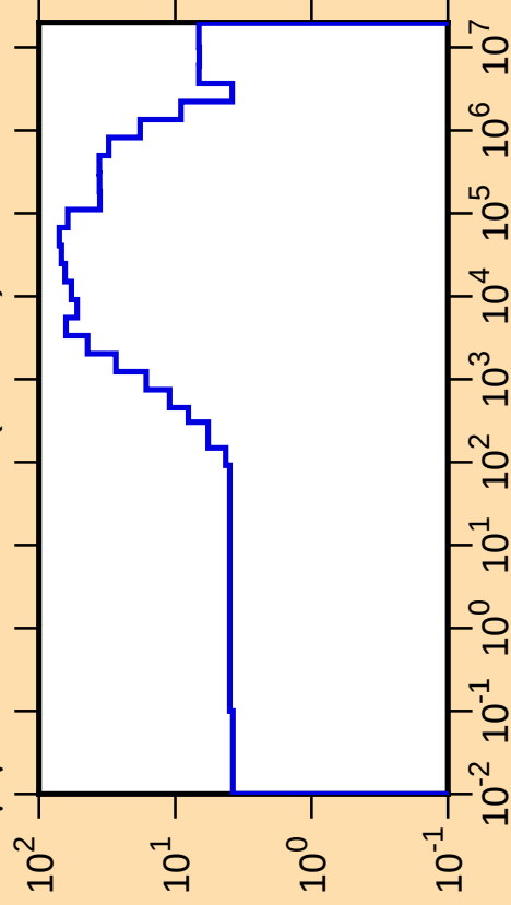
\Delta\mu/\mu vs. E for ^{131}\text{Cs}(\text{mt251})
