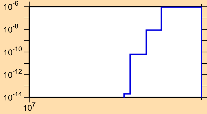
\sigma vs. E for ^{133}\text{Cs}(n,nd)
