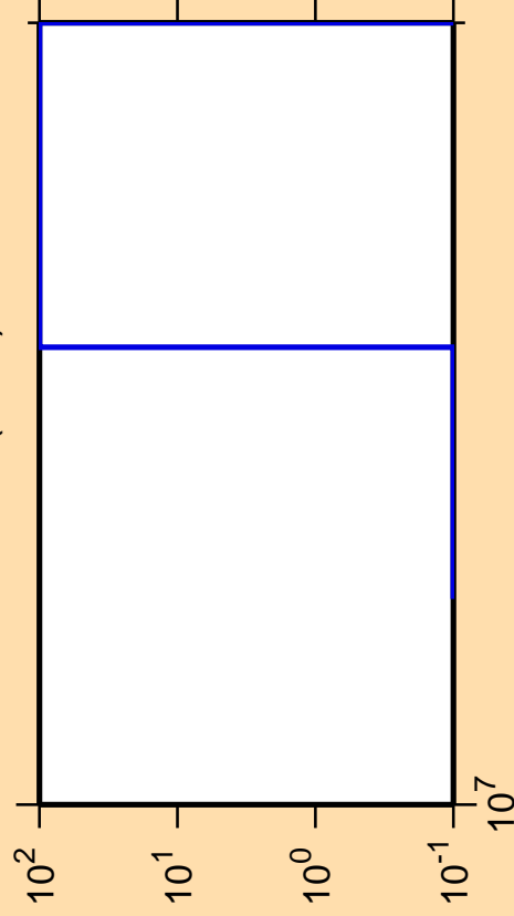
\Delta\sigma/\sigma vs. E for ^{133}\text{Cs}(n,nd)
