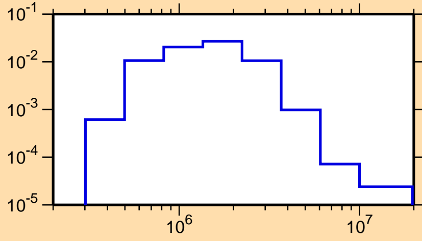
\sigma vs. E for ^{133}\text{Cs}(n,n_4)
