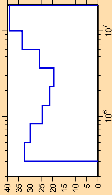
\Delta\sigma/\sigma vs. E for ^{133}\text{Cs}(n,n_4)
