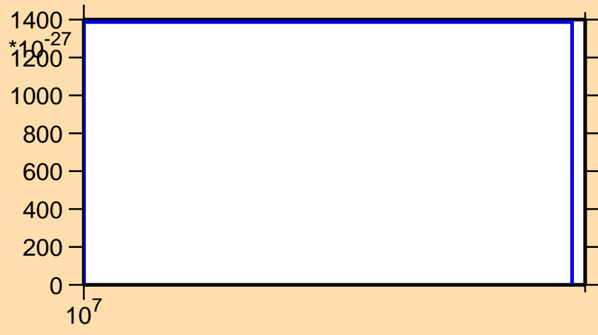
\sigma vs. E for ^{133}\text{Cs} (mt 11)
