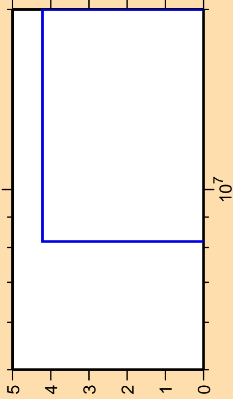
\Delta\sigma/\sigma vs. E for ^{133}\text{Cs}(n,2n\alpha)
