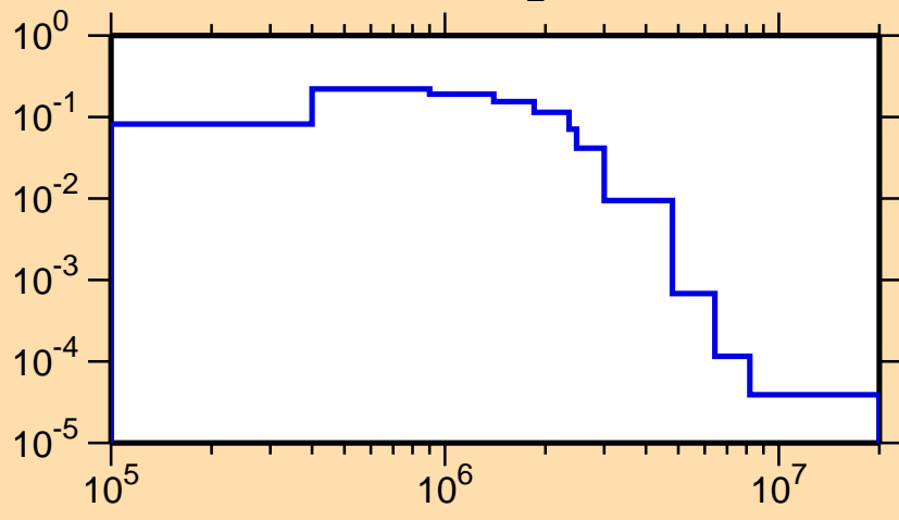
\sigma vs. E for ^{133}\text{Cs}(n,n_2)
