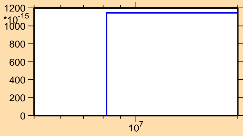
\sigma vs. E for ^{133}\text{Cs}(n,2n\alpha)
