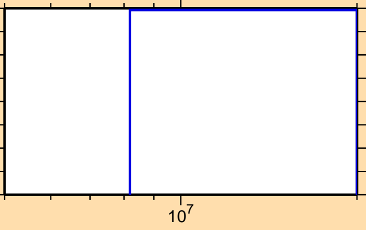
\sigma vs. E for ^{133}\text{Cs}(n,\text{nd})
