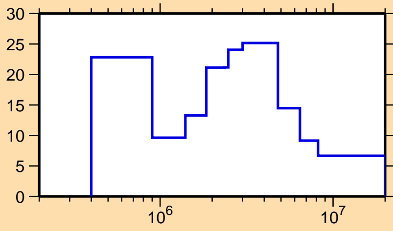
\Delta\sigma/\sigma vs. E for ^{134}\text{Cs}(n, el.)
