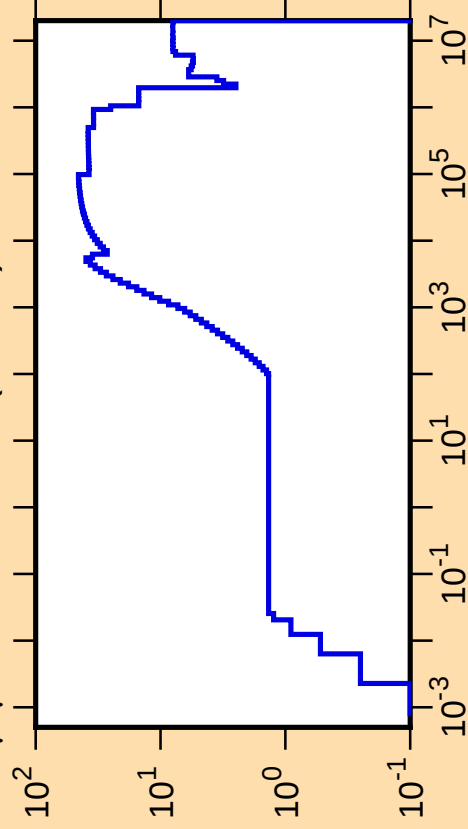
\Delta\mu/\mu vs. E for ^{135}\text{Cs}(\text{mt251})
