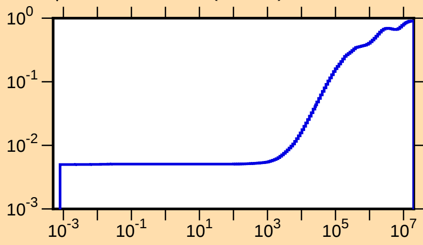
\mu vs. E for ^{135}\text{Cs}(\text{mt251})
