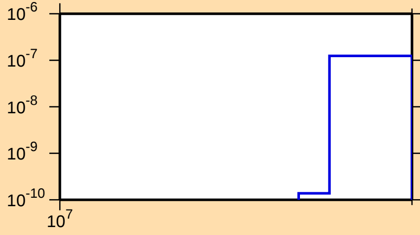
\sigma vs. E for ^{135}\text{Cs}(n,\text{nt})
