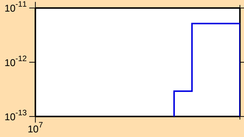
\sigma vs. E for ^{135}\text{Cs}(n,p\alpha)
