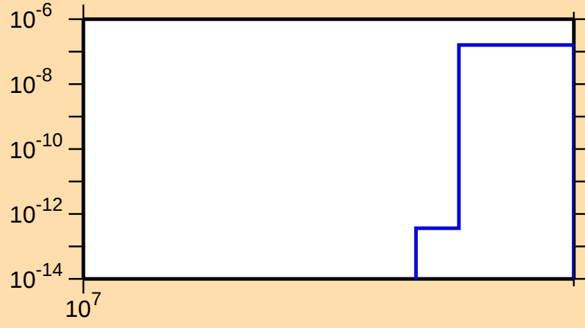
\sigma vs. E for ^{135}\text{Cs}(n,2np)
