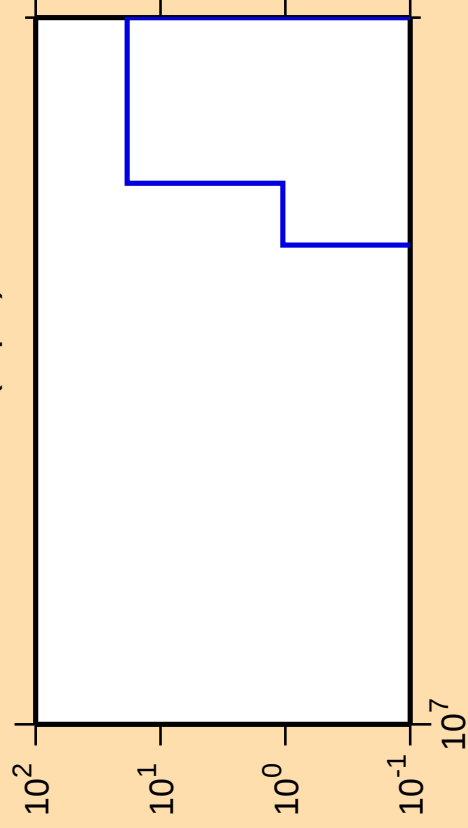
\Delta\sigma/\sigma vs. E for ^{135}\text{Cs}(n,p\alpha)
