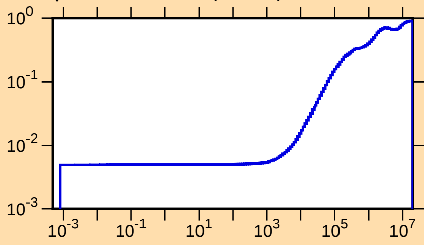
\mu vs. E for ^{136}\text{Cs}(\text{mt251})
