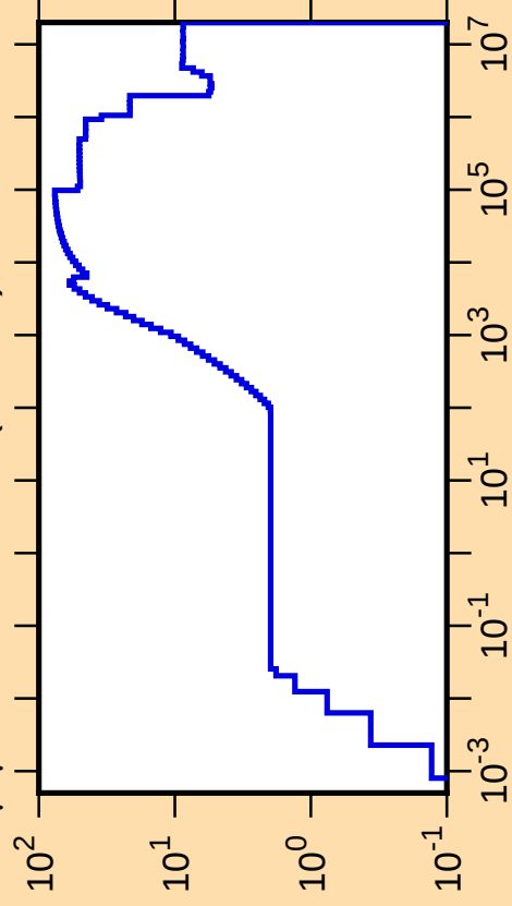
\Delta\mu/\mu vs. E for ^{136}\text{Cs}(\text{mt251})
