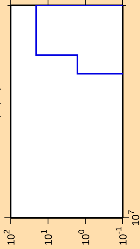
\Delta\sigma/\sigma vs. E for ^{136}\text{Cs}(n,p\alpha)
