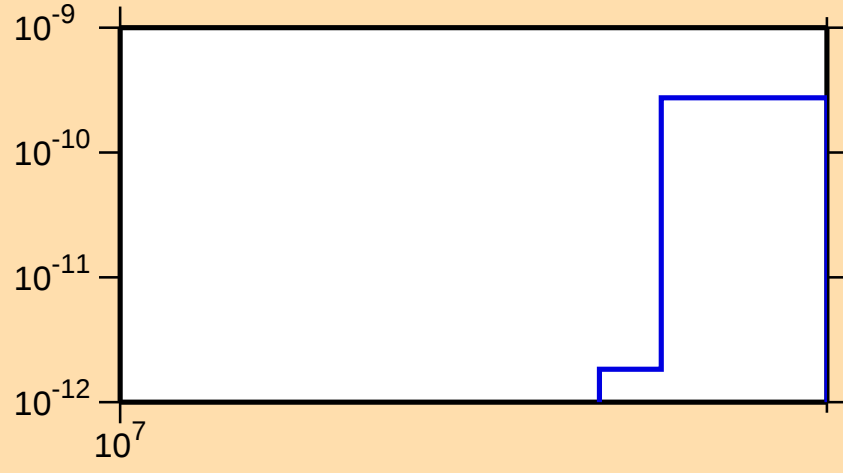
\sigma vs. E for ^{136}\text{Cs}(n,\text{He}3)
