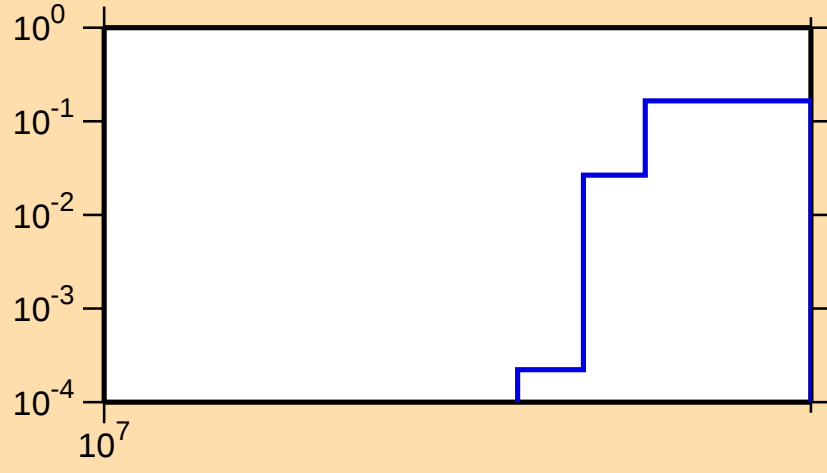
\sigma vs. E for ^{136}\text{Cs}(n,3n)
