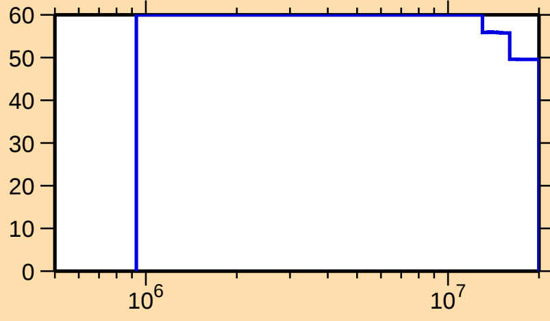
\Delta\sigma/\sigma vs. E for ^{136}\text{Cs}(n,p)
