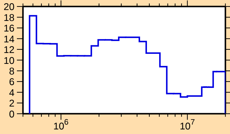
\Delta\sigma/\sigma vs. E for ^{136}\text{Cs}(n,\text{tot.})
