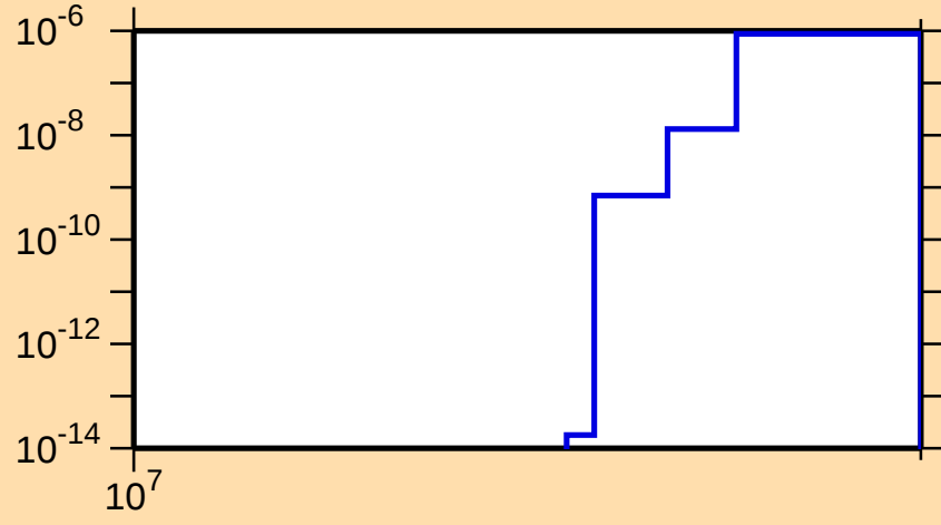
\sigma vs. E for ^{136}\text{Cs}(n,2np)
